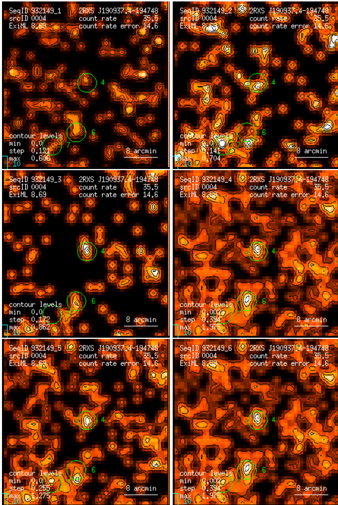
Figure 4: RASS 932149: detection 0004: band rate images, Gaussian filter: (1) PSPC channels 11 – 41, (2) 52 – 90, (3) 91 – 201, (4) 11 – 235, (5) 52 – 201, (6) 11 – 201. Broad band rates in counts/ks. Band rate contour levels in counts/ks/arcmin 2 .
