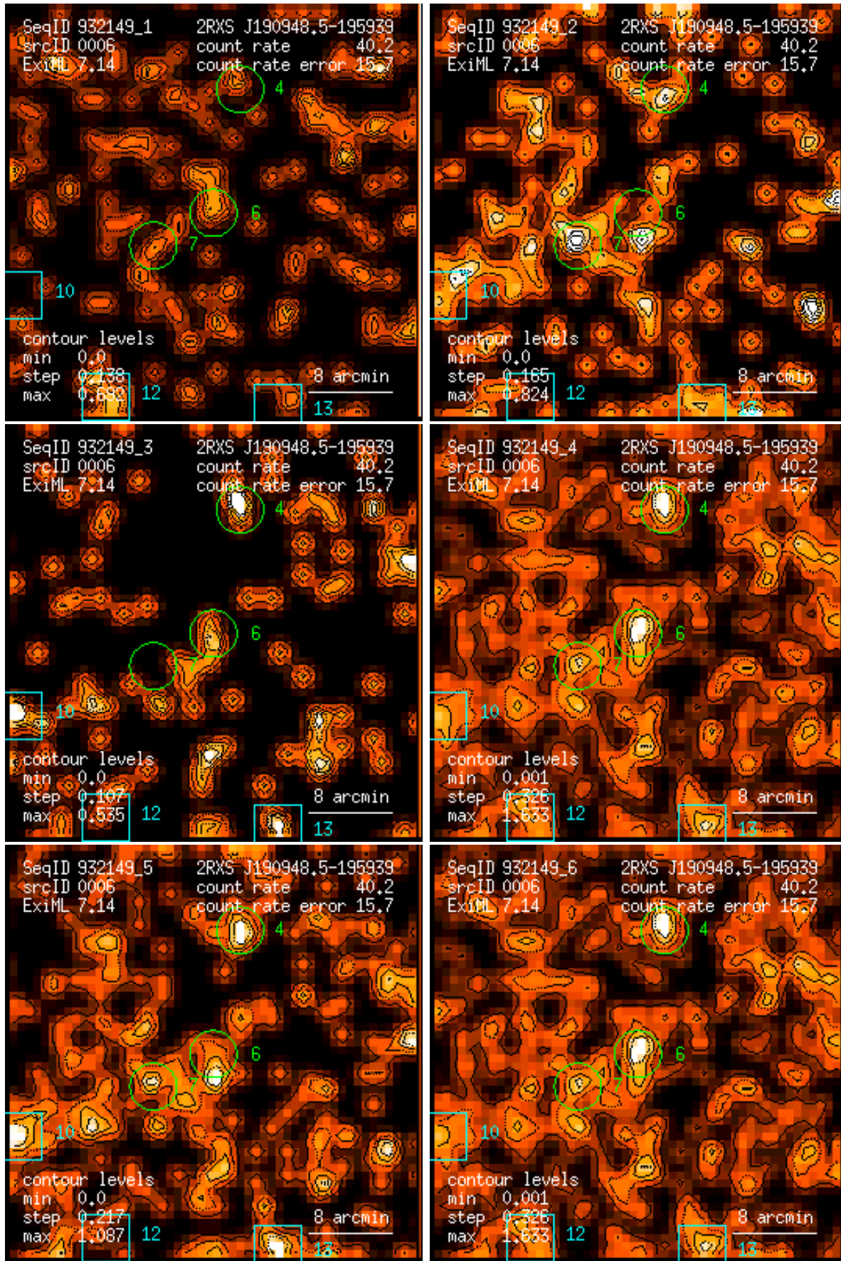
Figure 6: RASS 932149: detection 0006: band rate images, Gaussian filter: (1) PSPC channels 11 – 41, (2) 52 – 90, (3) 91 – 201, (4) 11 – 235, (5) 52 – 201, (6) 11 – 201. Broad band rates in counts/ks. Band rate contour levels in counts/ks/arcmin 2 .
