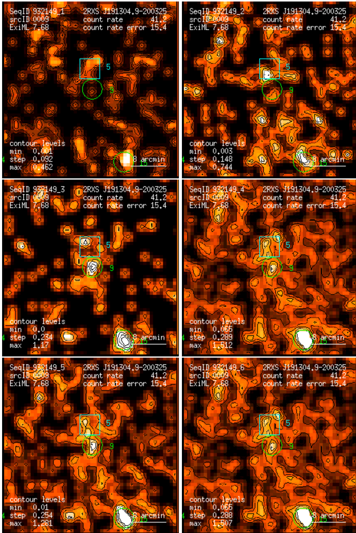
Figure 9: RASS 932149: detection 0009: band rate images, Gaussian filter: (1) PSPC channels 11 – 41, (2) 52 – 90, (3) 91 – 201, (4) 11 – 235, (5) 52 – 201, (6) 11 – 201. Broad band rates in counts/ks. Band rate contour levels in counts/ks/arcmin 2 .
