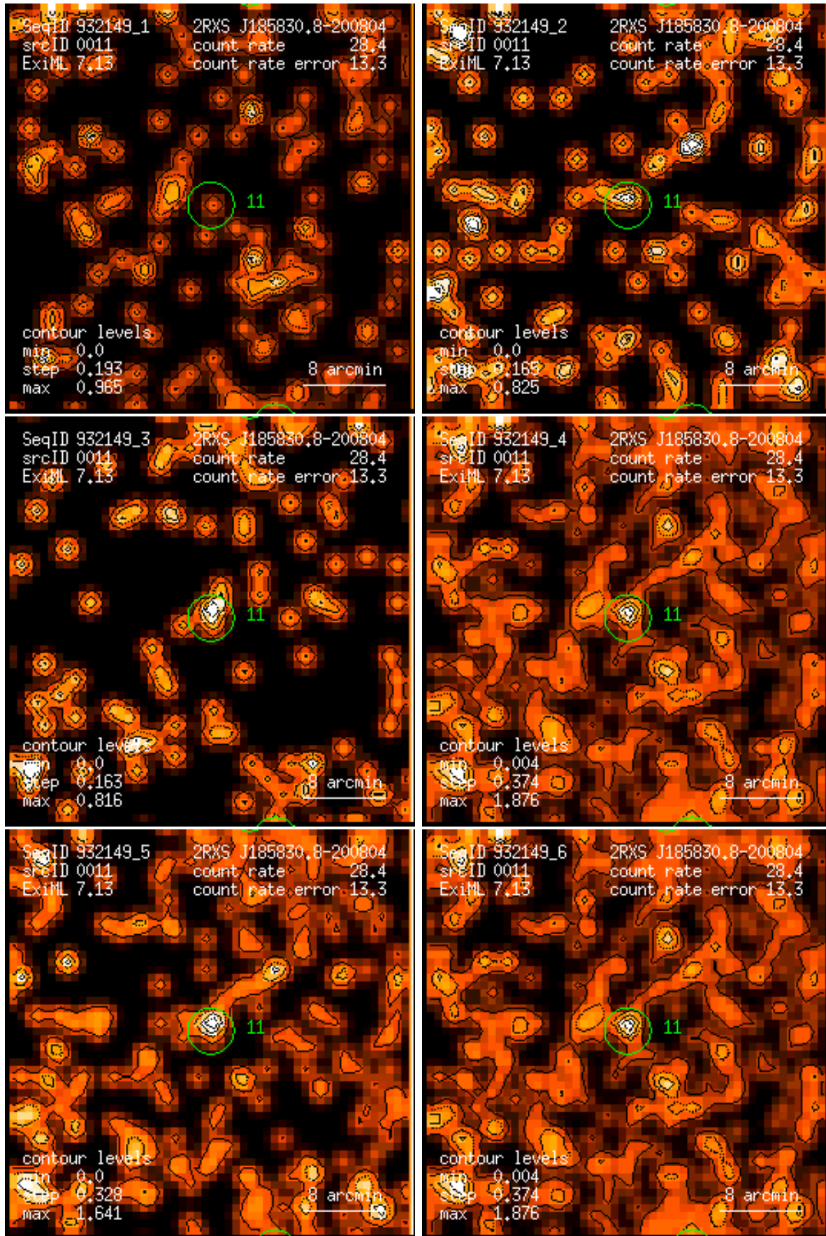
Figure 11: RASS 932149: detection 0011: band rate images, Gaussian filter: (1) PSPC channels 11 – 41, (2) 52 – 90, (3) 91 – 201, (4) 11 – 235, (5) 52 – 201, (6) 11 – 201. Broad band rates in counts/ks. Band rate contour levels in counts/ks/arcmin 2 .
