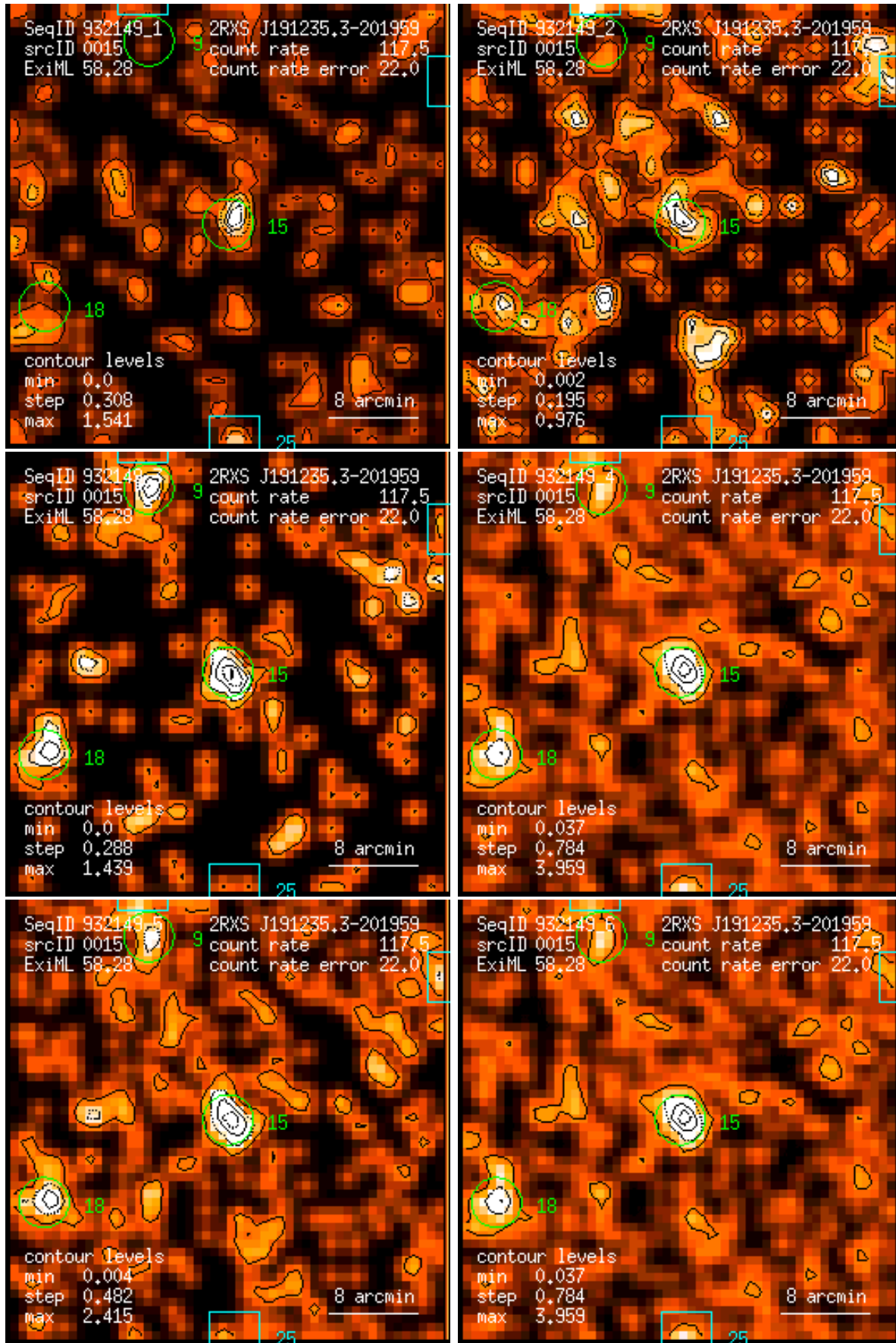
Figure 15: RASS 932149: detection 0015: band rate images, Gaussian filter: (1) PSPC channels 11 – 41, (2) 52 – 90, (3) 91 – 201, (4) 11 – 235, (5) 52 – 201, (6) 11 – 201. Broad band rates in counts/ks. Band rate contour levels in counts/ks/arcmin 2 .
