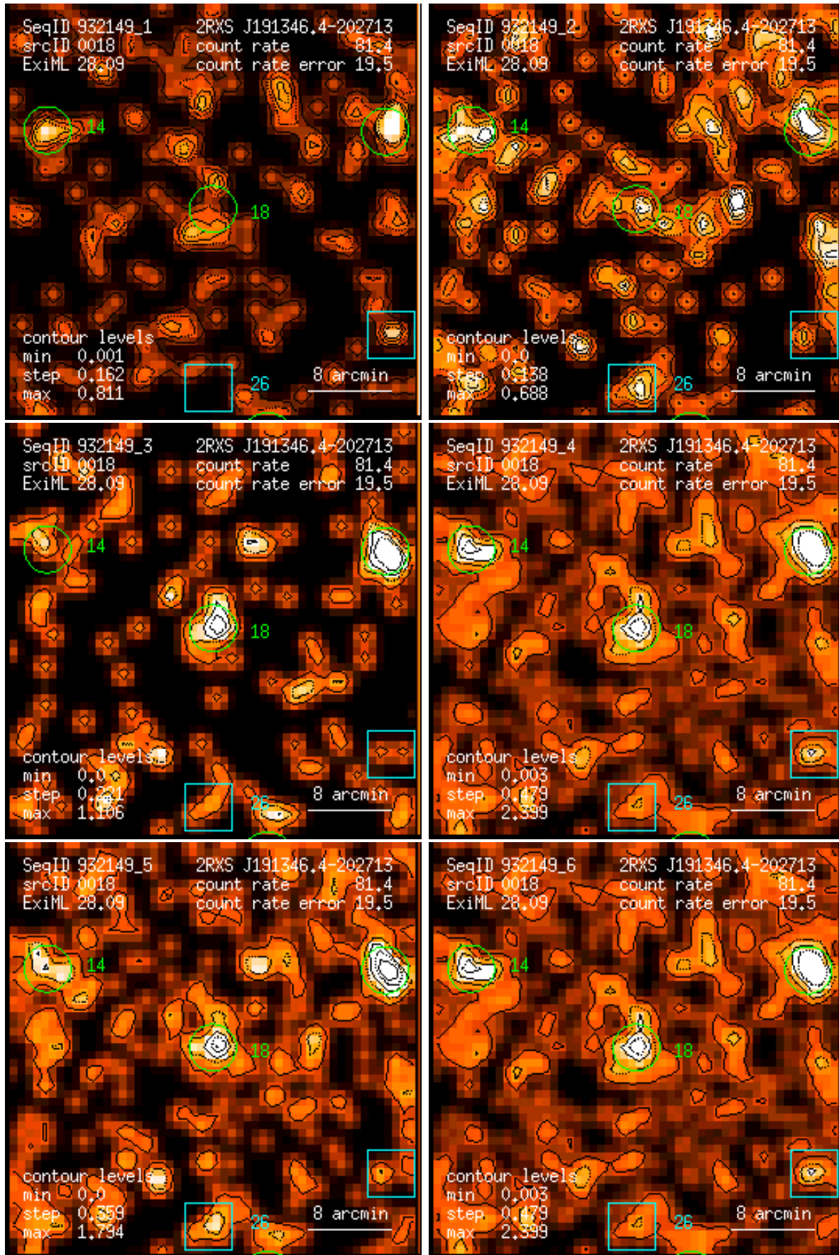
Figure 18: RASS 932149: detection 0018: band rate images, Gaussian filter: (1) PSPC channels 11 – 41, (2) 52 – 90, (3) 91 – 201, (4) 11 – 235, (5) 52 – 201, (6) 11 – 201. Broad band rates in counts/ks. Band rate contour levels in counts/ks/arcmin 2 .
