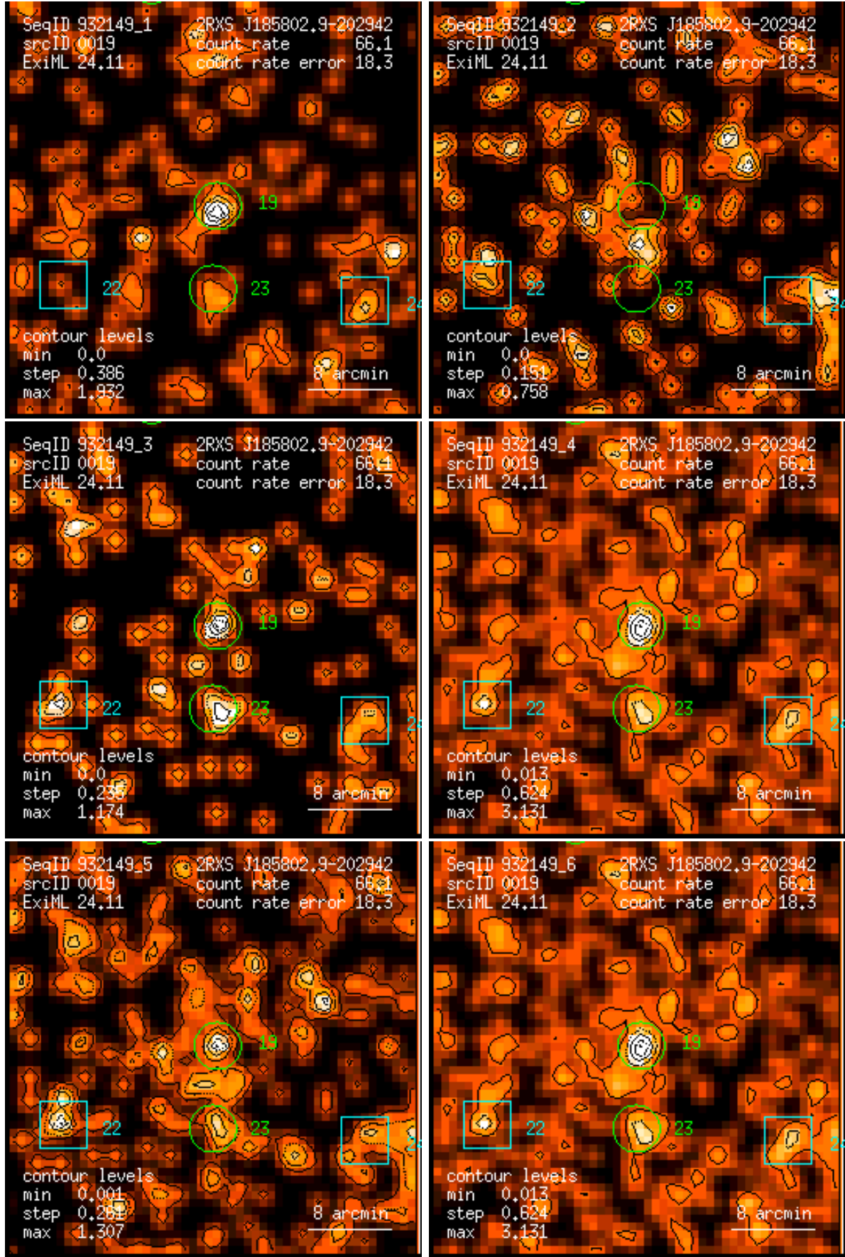
Figure 19: RASS 932149: detection 0019: band rate images, Gaussian filter: (1) PSPC channels 11 – 41, (2) 52 – 90, (3) 91 – 201, (4) 11 – 235, (5) 52 – 201, (6) 11 – 201. Broad band rates in counts/ks. Band rate contour levels in counts/ks/arcmin 2 .
