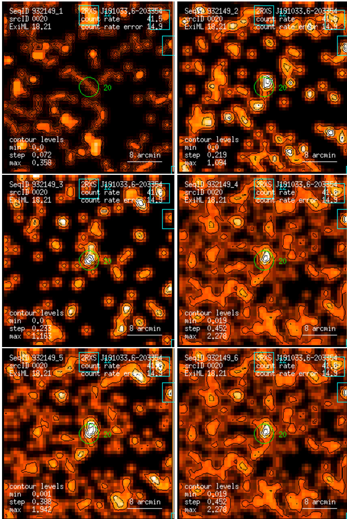
Figure 20: RASS 932149: detection 0020: band rate images, Gaussian filter: (1) PSPC channels 11 – 41, (2) 52 – 90, (3) 91 – 201, (4) 11 – 235, (5) 52 – 201, (6) 11 – 201. Broad band rates in counts/ks. Band rate contour levels in counts/ks/arcmin 2 .
