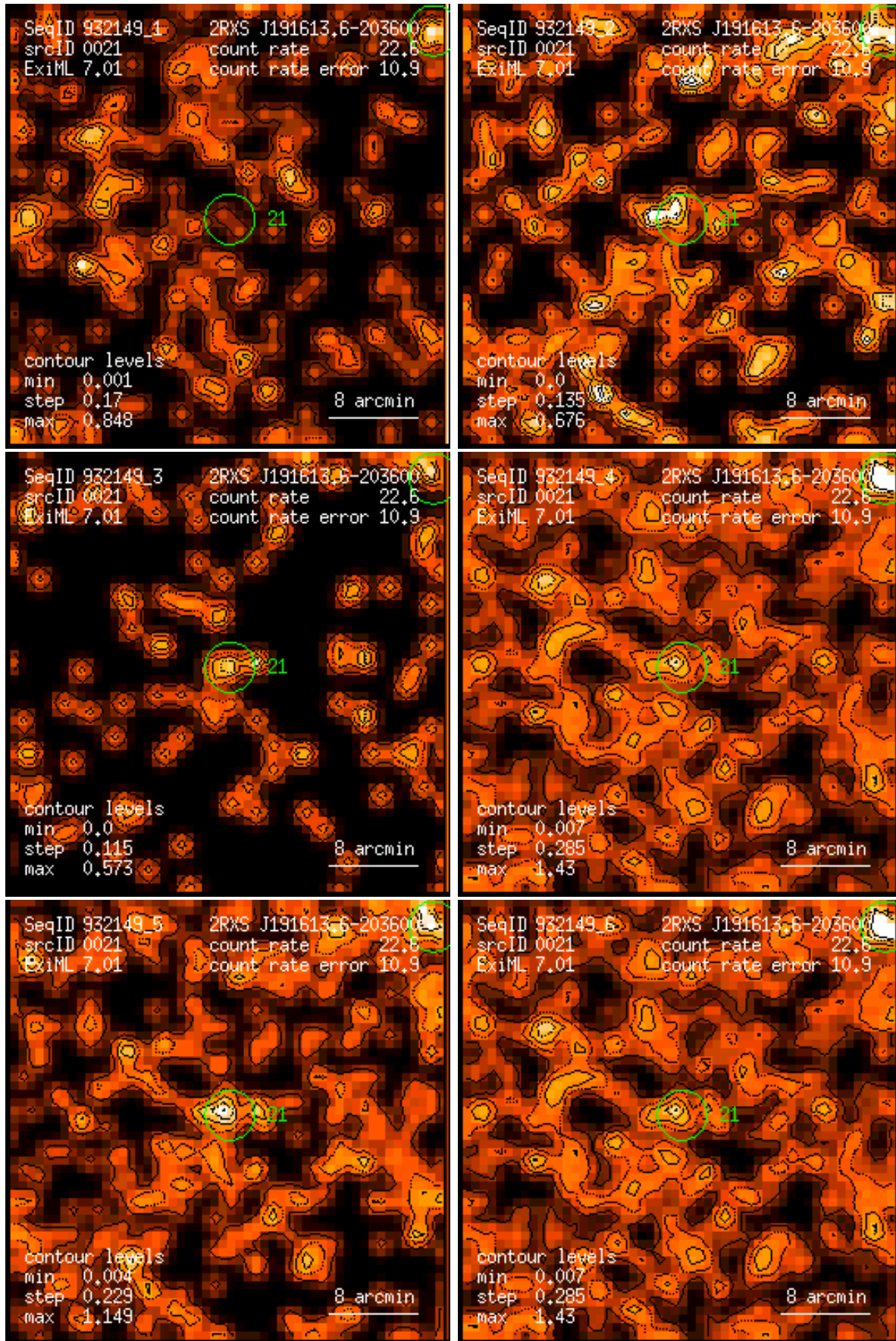
Figure 21: RASS 932149: detection 0021: band rate images, Gaussian filter: (1) PSPC channels 11 – 41, (2) 52 – 90, (3) 91 – 201, (4) 11 – 235, (5) 52 – 201, (6) 11 – 201. Broad band rates in counts/ks. Band rate contour levels in counts/ks/arcmin 2 .
