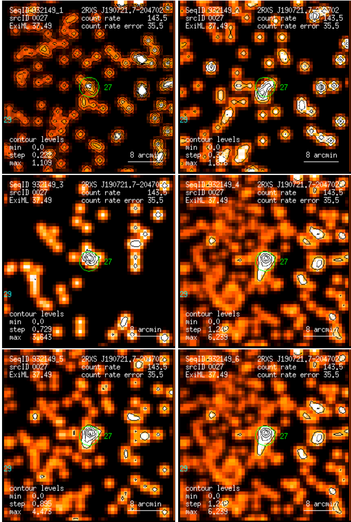
Figure 27: RASS 932149: detection 0027: band rate images, Gaussian filter: (1) PSPC channels 11 – 41, (2) 52 – 90, (3) 91 – 201, (4) 11 – 235, (5) 52 – 201, (6) 11 – 201. Broad band rates in counts/ks. Band rate contour levels in counts/ks/arcmin 2 .
