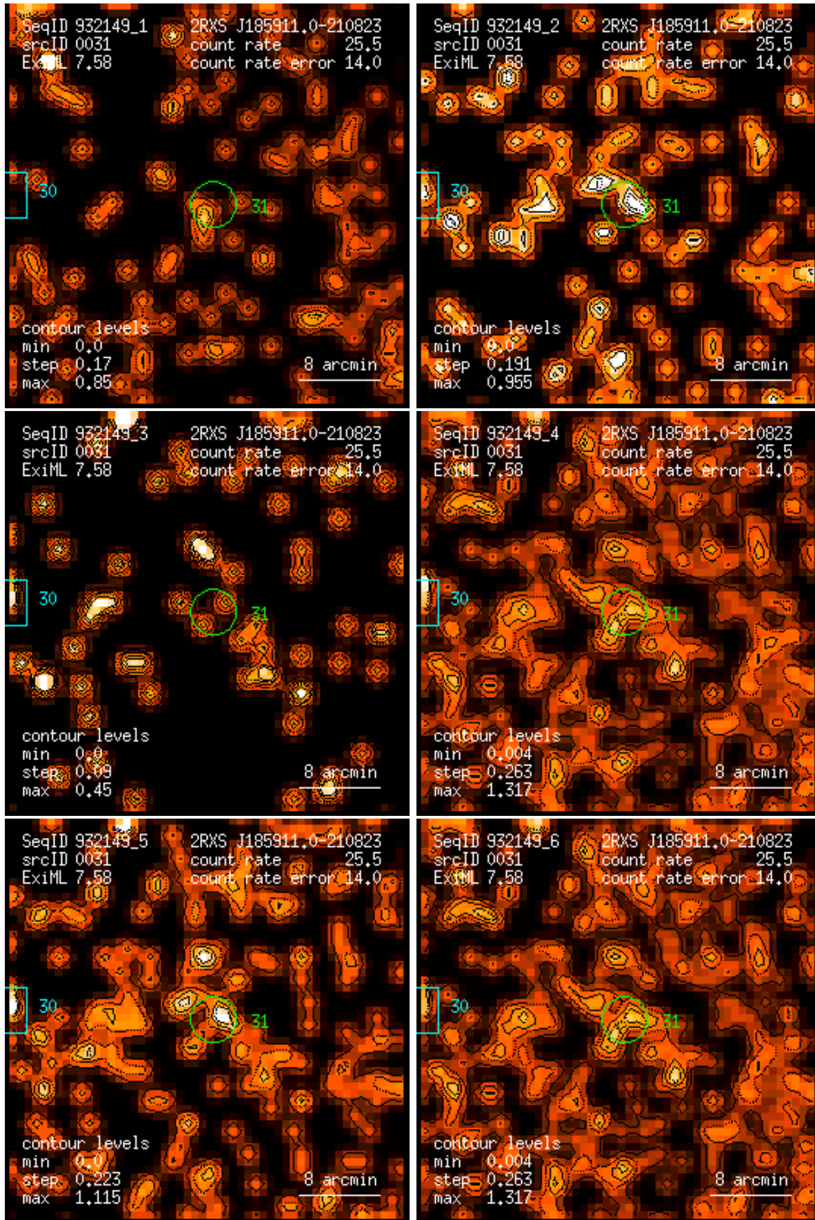
Figure 31: RASS 932149: detection 0031: band rate images, Gaussian filter: (1) PSPC channels 11 – 41, (2) 52 – 90, (3) 91 – 201, (4) 11 – 235, (5) 52 – 201, (6) 11 – 201. Broad band rates in counts/ks. Band rate contour levels in counts/ks/arcmin 2 .
