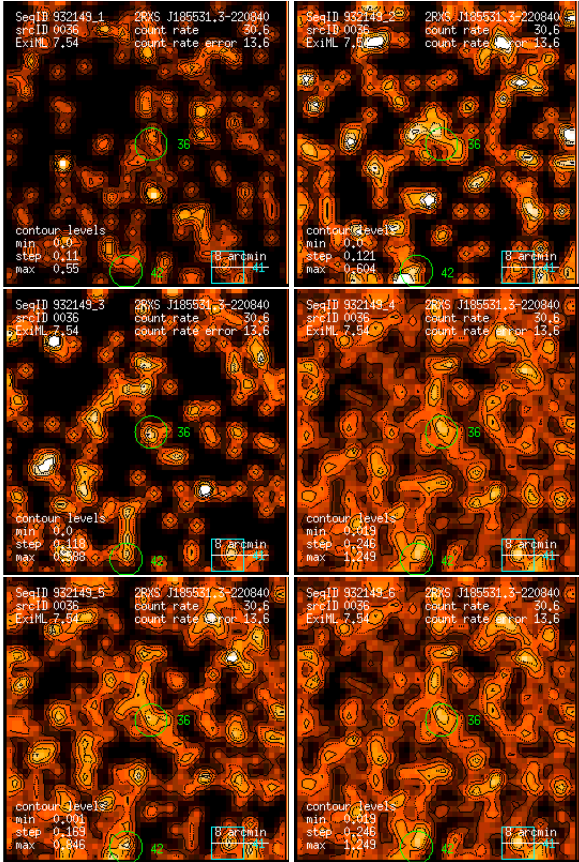
Figure 36: RASS 932149: detection 0036: band rate images, Gaussian filter: (1) PSPC channels 11 – 41, (2) 52 – 90, (3) 91 – 201, (4) 11 – 235, (5) 52 – 201, (6) 11 – 201. Broad band rates in counts/ks. Band rate contour levels in counts/ks/arcmin 2 .
