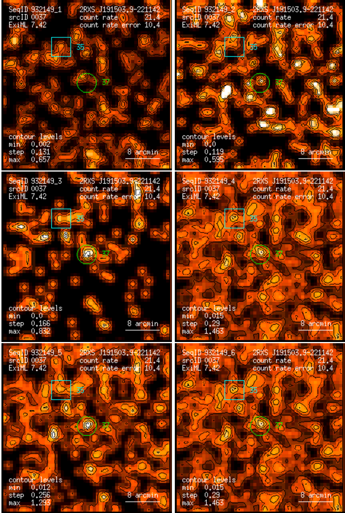
Figure 37: RASS 932149: detection 0037: band rate images, Gaussian filter: (1) PSPC channels 11 – 41, (2) 52 – 90, (3) 91 – 201, (4) 11 – 235, (5) 52 – 201, (6) 11 – 201. Broad band rates in counts/ks. Band rate contour levels in counts/ks/arcmin 2 .
