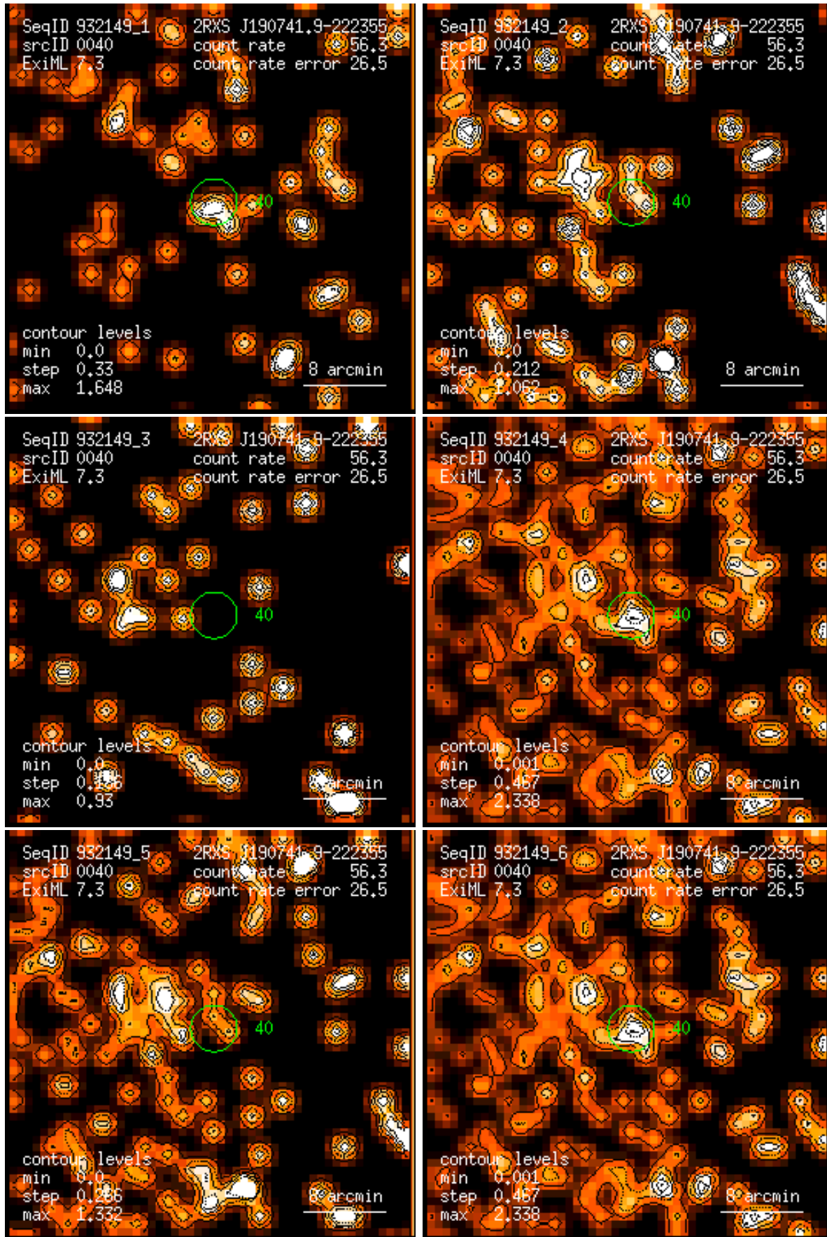
Figure 40: RASS 932149: detection 0040: band rate images, Gaussian filter: (1) PSPC channels 11 – 41, (2) 52 – 90, (3) 91 – 201, (4) 11 – 235, (5) 52 – 201, (6) 11 – 201. Broad band rates in counts/ks. Band rate contour levels in counts/ks/arcmin 2 .
