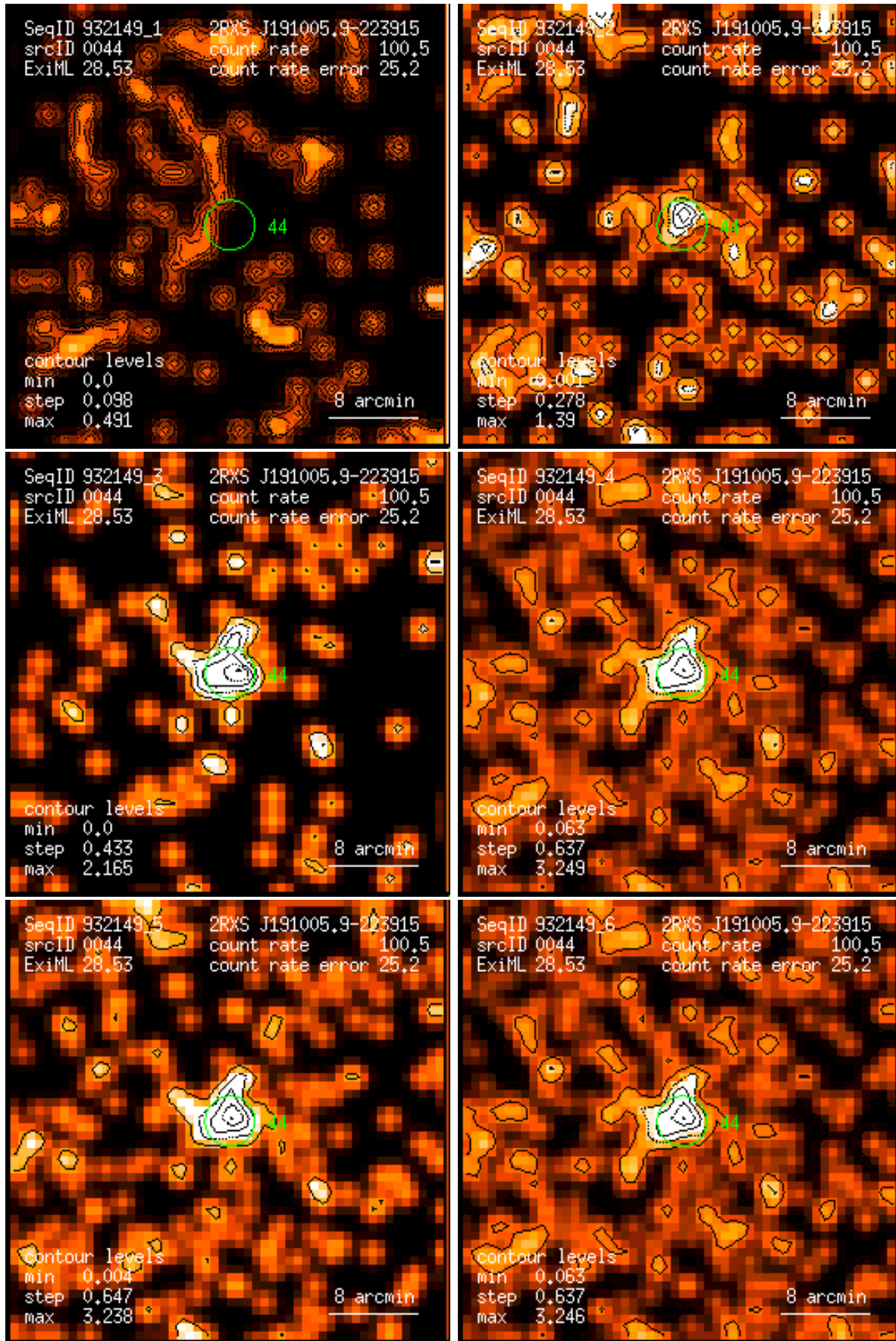
Figure 44: RASS 932149: detection 0044: band rate images, Gaussian filter: (1) PSPC channels 11 – 41, (2) 52 – 90, (3) 91 – 201, (4) 11 – 235, (5) 52 – 201, (6) 11 – 201. Broad band rates in counts/ks. Band rate contour levels in counts/ks/arcmin 2 .
