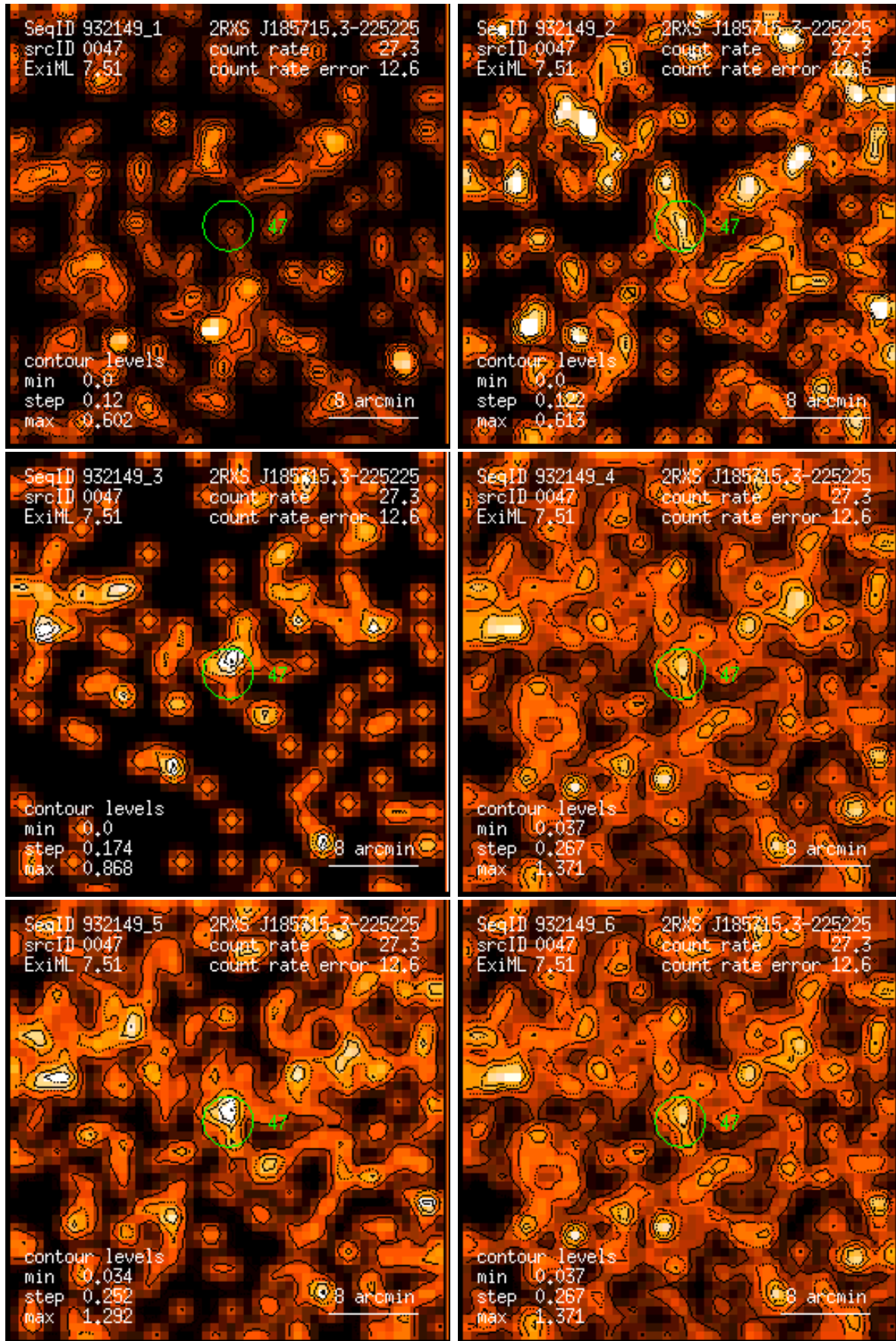
Figure 47: RASS 932149: detection 0047: band rate images, Gaussian filter: (1) PSPC channels 11 – 41, (2) 52 – 90, (3) 91 – 201, (4) 11 – 235, (5) 52 – 201, (6) 11 – 201. Broad band rates in counts/ks. Band rate contour levels in counts/ks/arcmin 2 .
