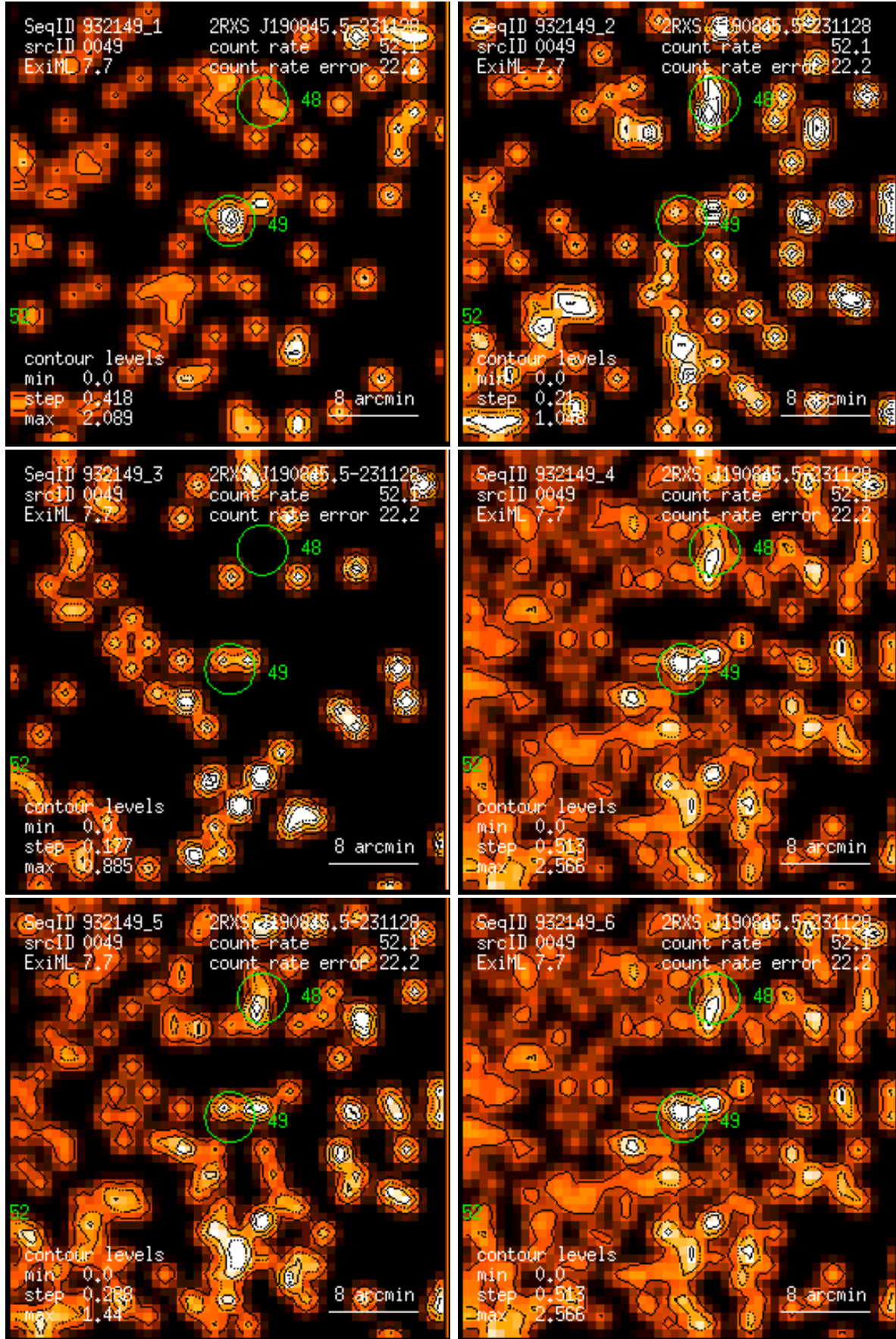
Figure 49: RASS 932149: detection 0049: band rate images, Gaussian filter: (1) PSPC channels 11 – 41, (2) 52 – 90, (3) 91 – 201, (4) 11 – 235, (5) 52 – 201, (6) 11 – 201. Broad band rates in counts/ks. Band rate contour levels in counts/ks/arcmin 2 .
