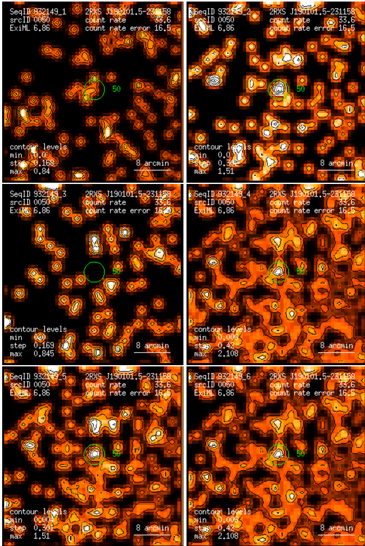
Figure 50: RASS 932149: detection 0050: band rate images, Gaussian filter: (1) PSPC channels 11 – 41, (2) 52 – 90, (3) 91 – 201, (4) 11 – 235, (5) 52 – 201, (6) 11 – 201. Broad band rates in counts/ks. Band rate contour levels in counts/ks/arcmin 2 .
