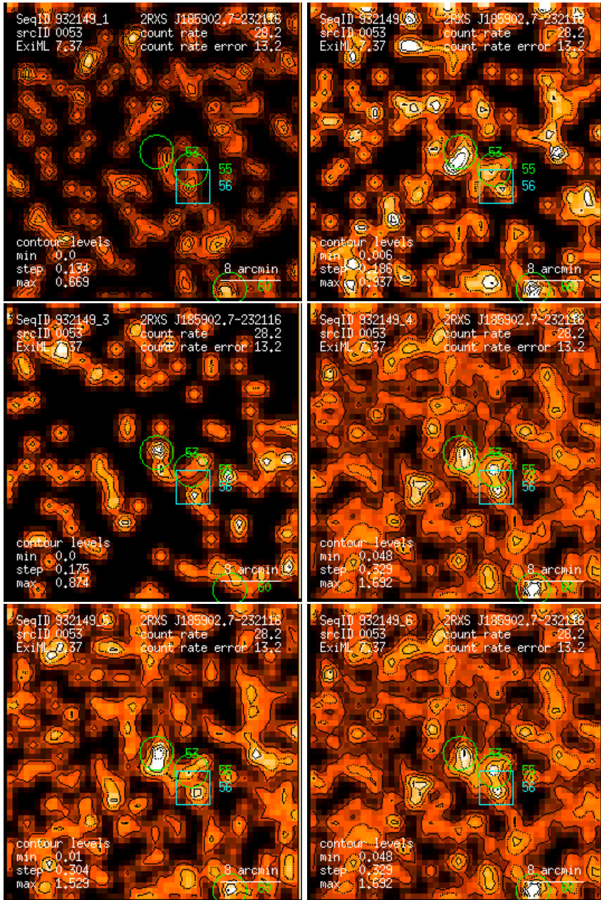
Figure 53: RASS 932149: detection 0053: band rate images, Gaussian filter: (1) PSPC channels 11 – 41, (2) 52 – 90, (3) 91 – 201, (4) 11 – 235, (5) 52 – 201, (6) 11 – 201. Broad band rates in counts/ks. Band rate contour levels in counts/ks/arcmin 2 .
