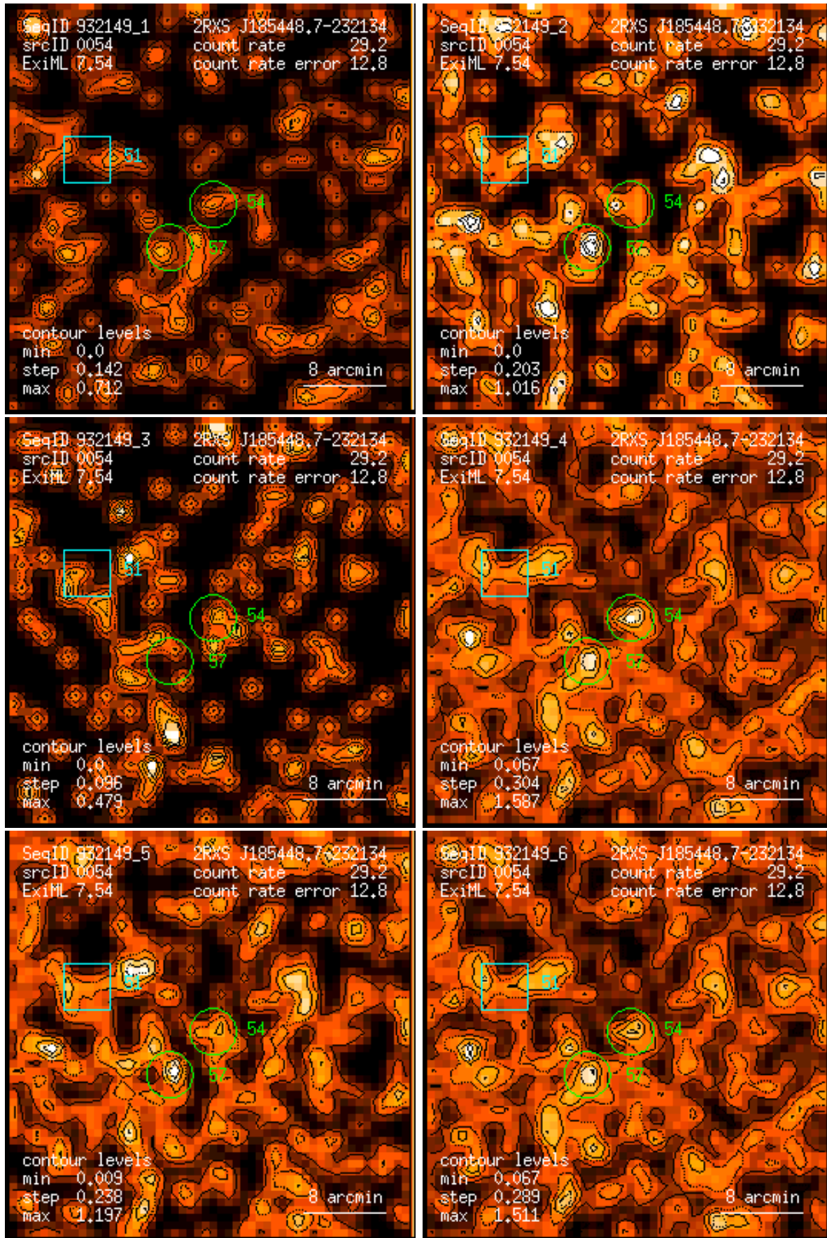
Figure 54: RASS 932149: detection 0054: band rate images, Gaussian filter: (1) PSPC channels 11 – 41, (2) 52 – 90, (3) 91 – 201, (4) 11 – 235, (5) 52 – 201, (6) 11 – 201. Broad band rates in counts/ks. Band rate contour levels in counts/ks/arcmin 2 .
