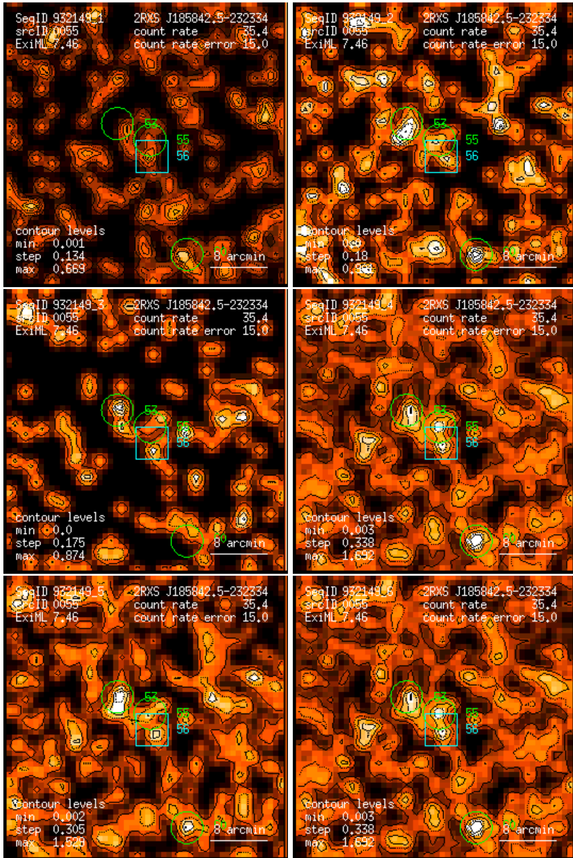
Figure 55: RASS 932149: detection 0055: band rate images, Gaussian filter: (1) PSPC channels 11 – 41, (2) 52 – 90, (3) 91 – 201, (4) 11 – 235, (5) 52 – 201, (6) 11 – 201. Broad band rates in counts/ks. Band rate contour levels in counts/ks/arcmin 2 .
