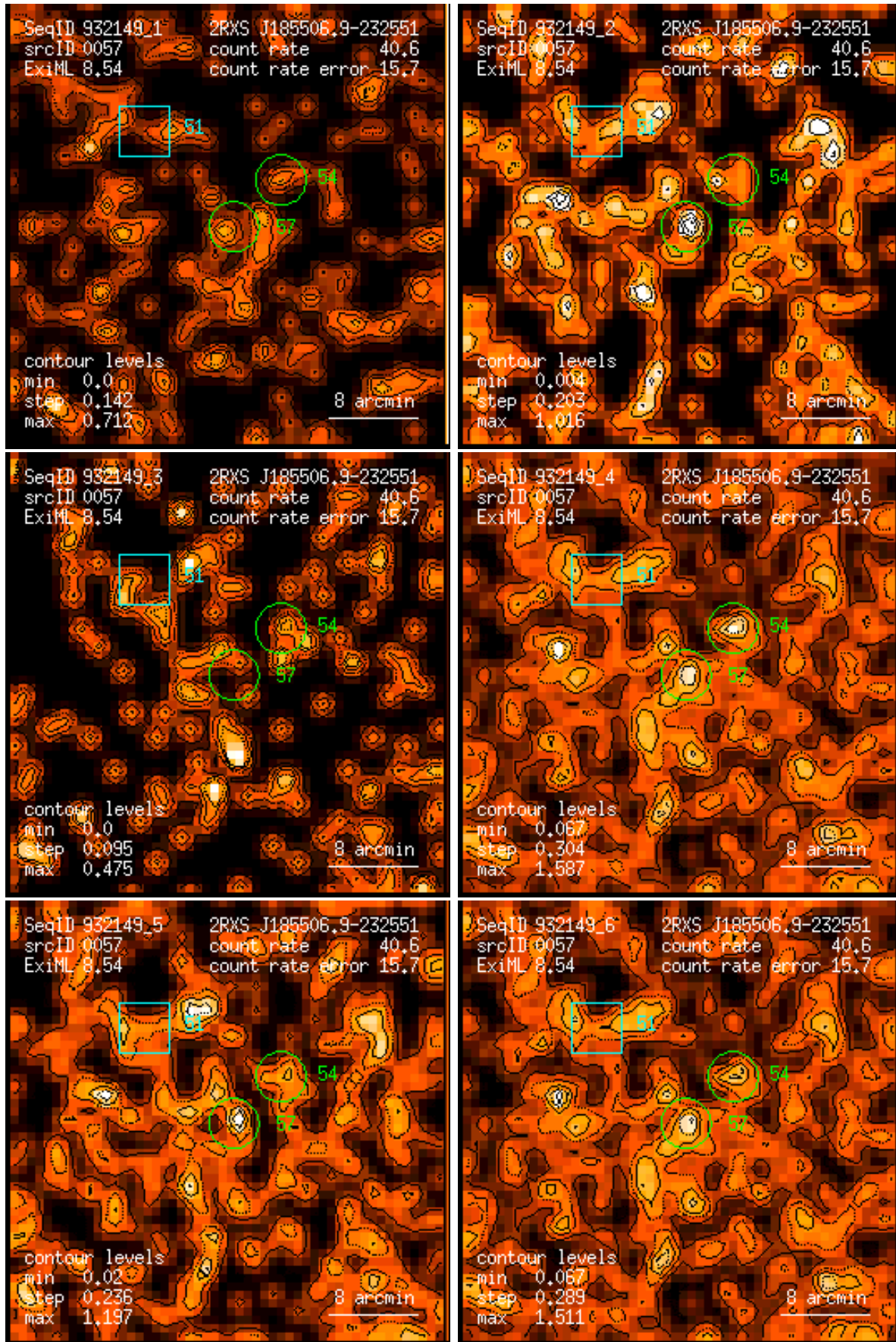
Figure 57: RASS 932149: detection 0057: band rate images, Gaussian filter: (1) PSPC channels 11 – 41, (2) 52 – 90, (3) 91 – 201, (4) 11 – 235, (5) 52 – 201, (6) 11 – 201. Broad band rates in counts/ks. Band rate contour levels in counts/ks/arcmin 2 .
