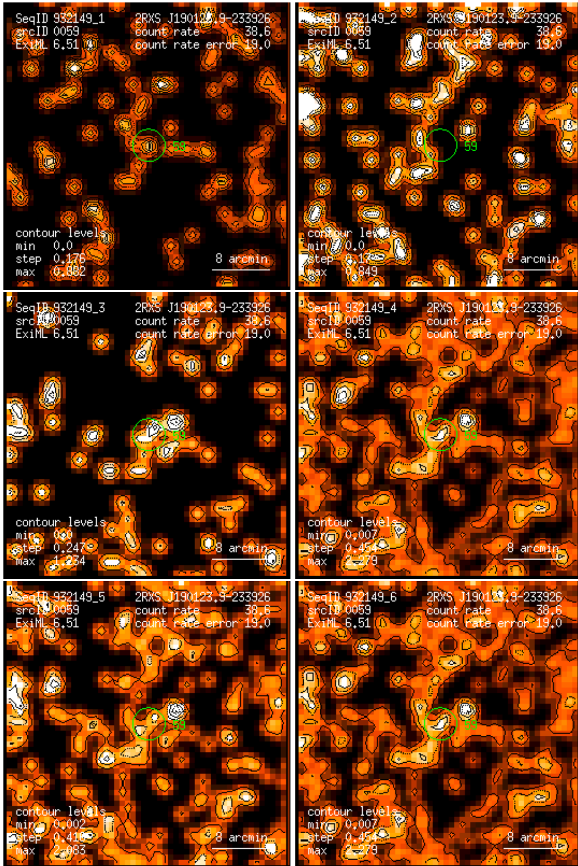
Figure 59: RASS 932149: detection 0059: band rate images, Gaussian filter: (1) PSPC channels 11 – 41, (2) 52 – 90, (3) 91 – 201, (4) 11 – 235, (5) 52 – 201, (6) 11 – 201. Broad band rates in counts/ks. Band rate contour levels in counts/ks/arcmin 2 .
