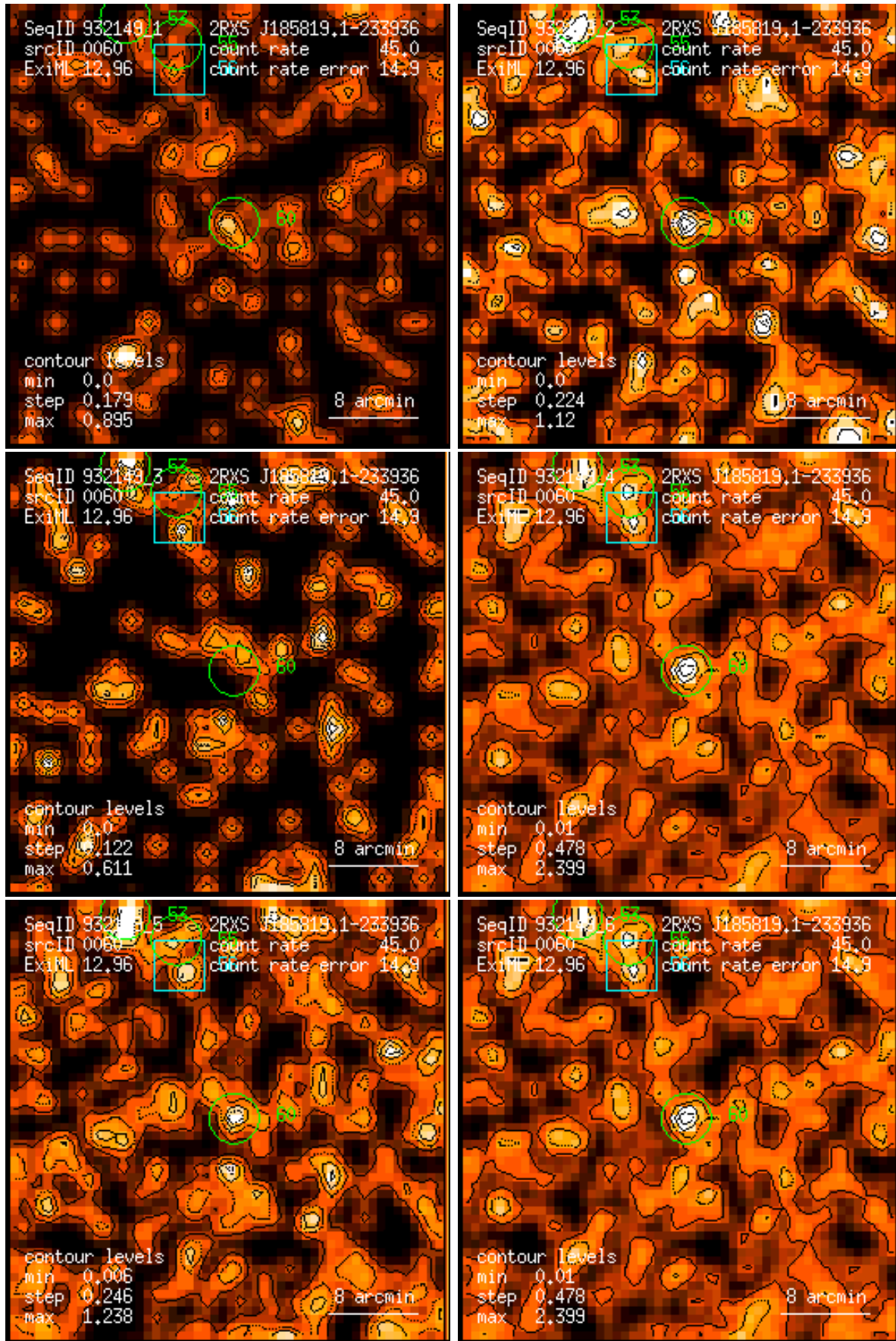
Figure 60: RASS 932149: detection 0060: band rate images, Gaussian filter: (1) PSPC channels 11 – 41, (2) 52 – 90, (3) 91 – 201, (4) 11 – 235, (5) 52 – 201, (6) 11 – 201. Broad band rates in counts/ks. Band rate contour levels in counts/ks/arcmin 2 .
