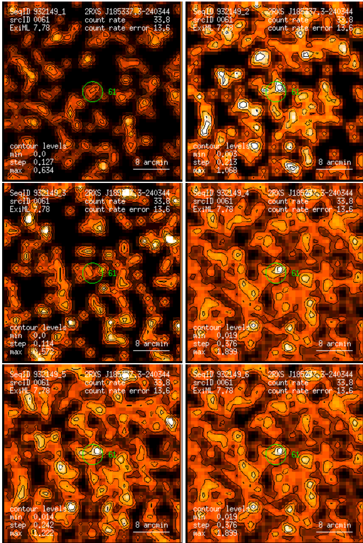
Figure 61: RASS 932149: detection 0061: band rate images, Gaussian filter: (1) PSPC channels 11 – 41, (2) 52 – 90, (3) 91 – 201, (4) 11 – 235, (5) 52 – 201, (6) 11 – 201. Broad band rates in counts/ks. Band rate contour levels in counts/ks/arcmin 2 .
