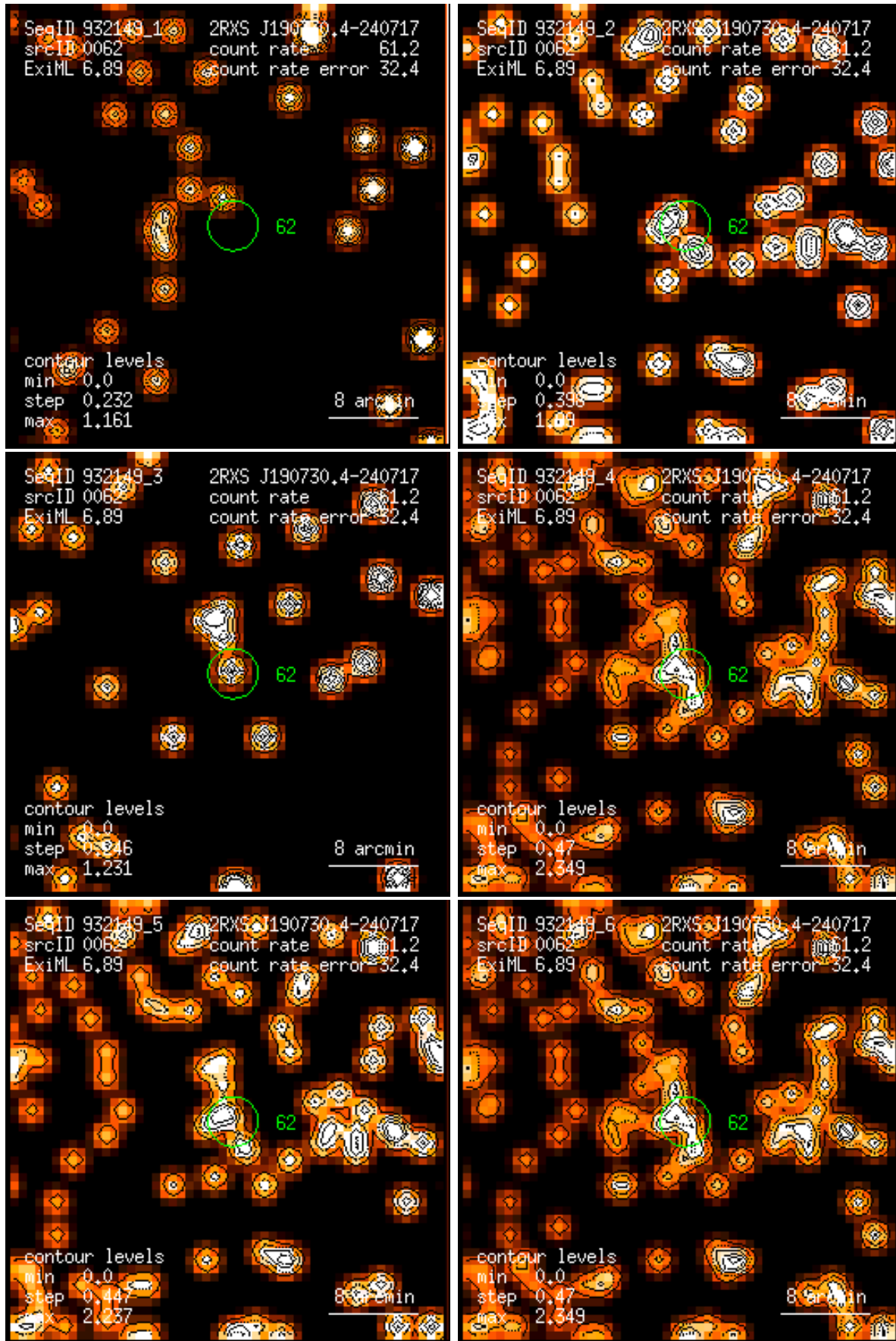
Figure 62: RASS 932149: detection 0062: band rate images, Gaussian filter: (1) PSPC channels 11 – 41, (2) 52 – 90, (3) 91 – 201, (4) 11 – 235, (5) 52 – 201, (6) 11 – 201. Broad band rates in counts/ks. Band rate contour levels in counts/ks/arcmin 2 .
