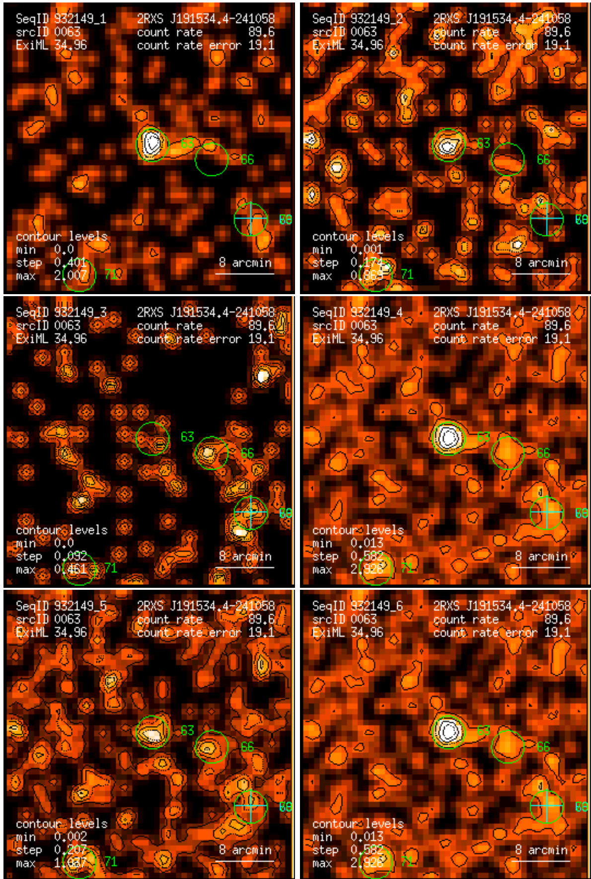
Figure 63: RASS 932149: detection 0063: band rate images, Gaussian filter: (1) PSPC channels 11 – 41, (2) 52 – 90, (3) 91 – 201, (4) 11 – 235, (5) 52 – 201, (6) 11 – 201. Broad band rates in counts/ks. Band rate contour levels in counts/ks/arcmin 2 .
