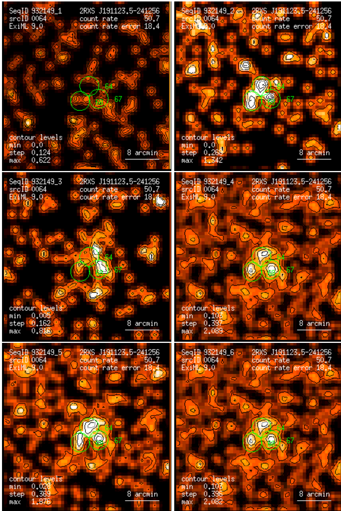
Figure 64: RASS 932149: detection 0064: band rate images, Gaussian filter: (1) PSPC channels 11 – 41, (2) 52 – 90, (3) 91 – 201, (4) 11 – 235, (5) 52 – 201, (6) 11 – 201. Broad band rates in counts/ks. Band rate contour levels in counts/ks/arcmin 2 .
