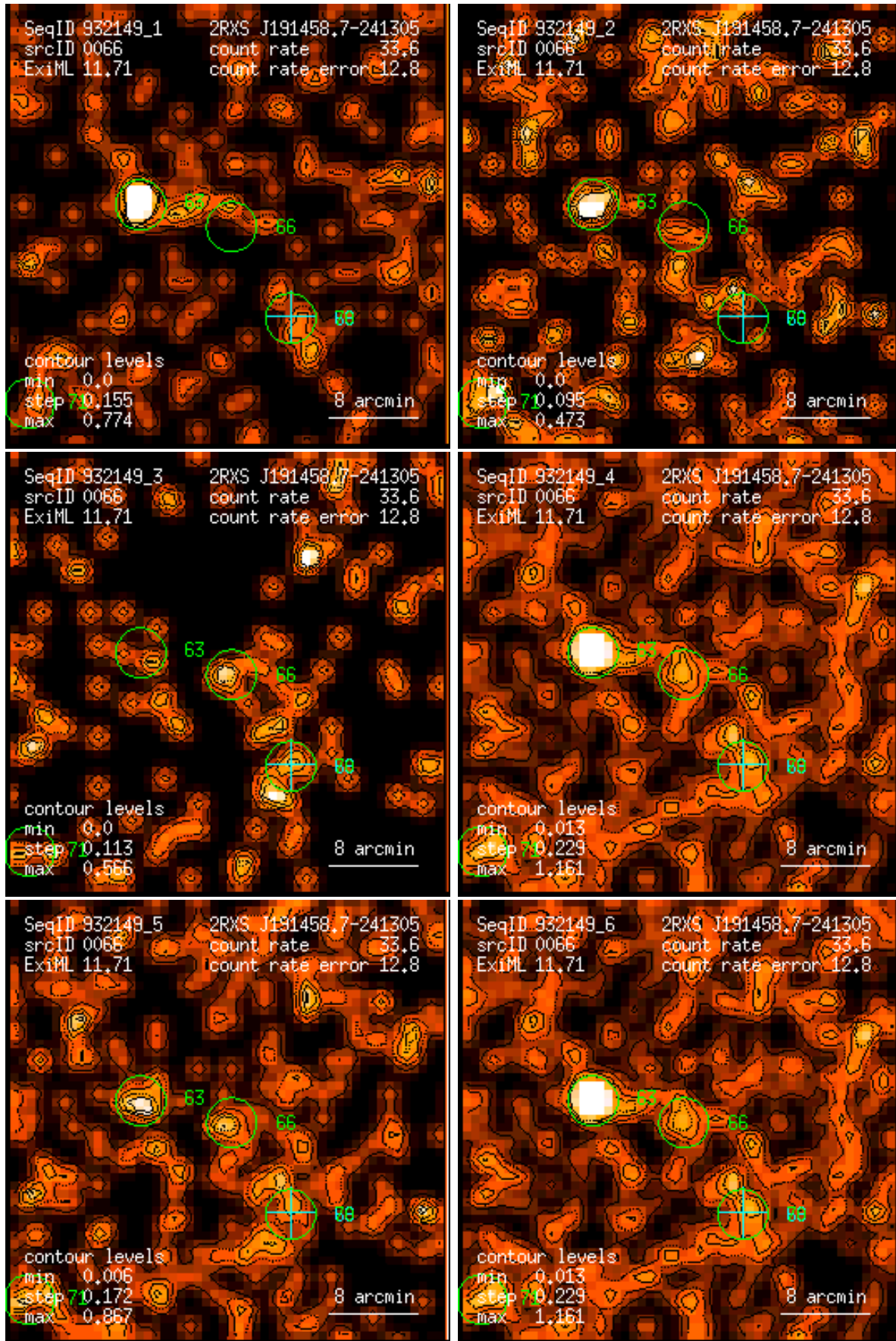
Figure 66: RASS 932149: detection 0066: band rate images, Gaussian filter: (1) PSPC channels 11 – 41, (2) 52 – 90, (3) 91 – 201, (4) 11 – 235, (5) 52 – 201, (6) 11 – 201. Broad band rates in counts/ks. Band rate contour levels in counts/ks/arcmin 2 .
