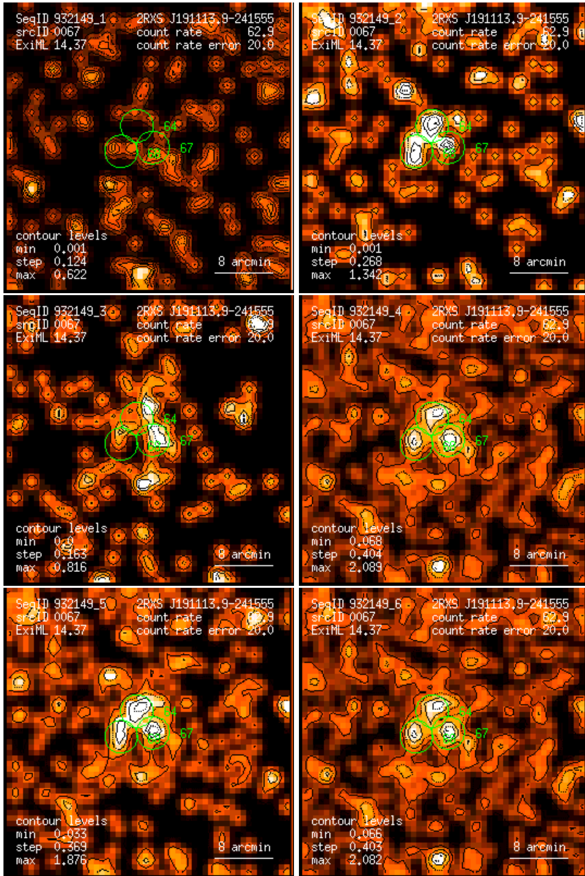
Figure 67: RASS 932149: detection 0067: band rate images, Gaussian filter: (1) PSPC channels 11 – 41, (2) 52 – 90, (3) 91 – 201, (4) 11 – 235, (5) 52 – 201, (6) 11 – 201. Broad band rates in counts/ks. Band rate contour levels in counts/ks/arcmin 2 .
