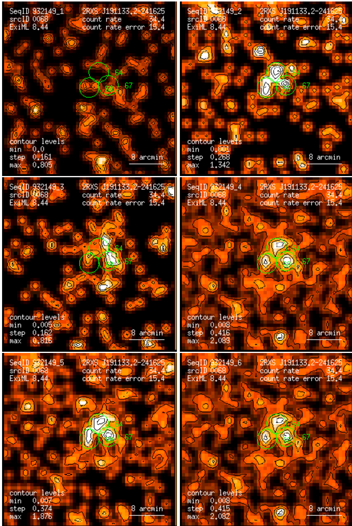
Figure 68: RASS 932149: detection 0068: band rate images, Gaussian filter: (1) PSPC channels 11 – 41, (2) 52 – 90, (3) 91 – 201, (4) 11 – 235, (5) 52 – 201, (6) 11 – 201. Broad band rates in counts/ks. Band rate contour levels in counts/ks/arcmin 2 .
