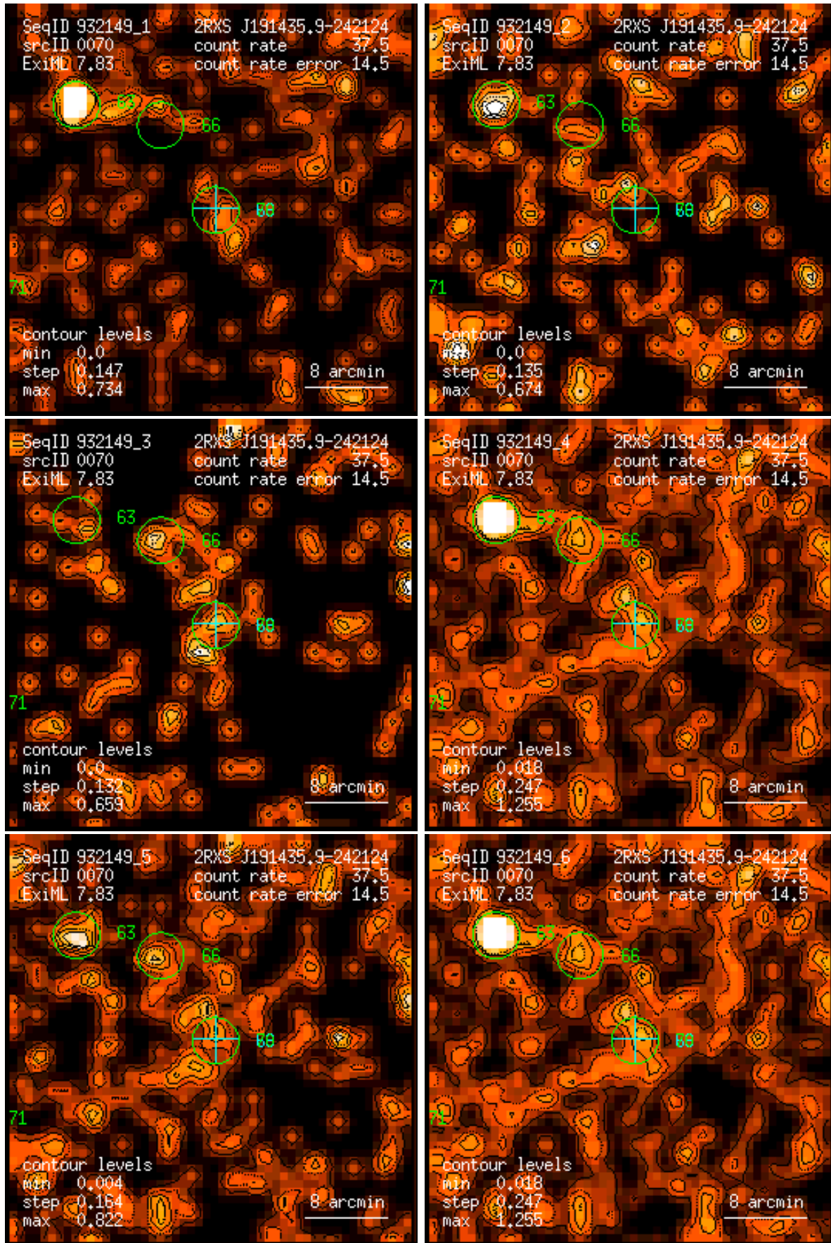
Figure 70: RASS 932149: detection 0070: band rate images, Gaussian filter: (1) PSPC channels 11 – 41, (2) 52 – 90, (3) 91 – 201, (4) 11 – 235, (5) 52 – 201, (6) 11 – 201. Broad band rates in counts/ks. Band rate contour levels in counts/ks/arcmin 2 .
