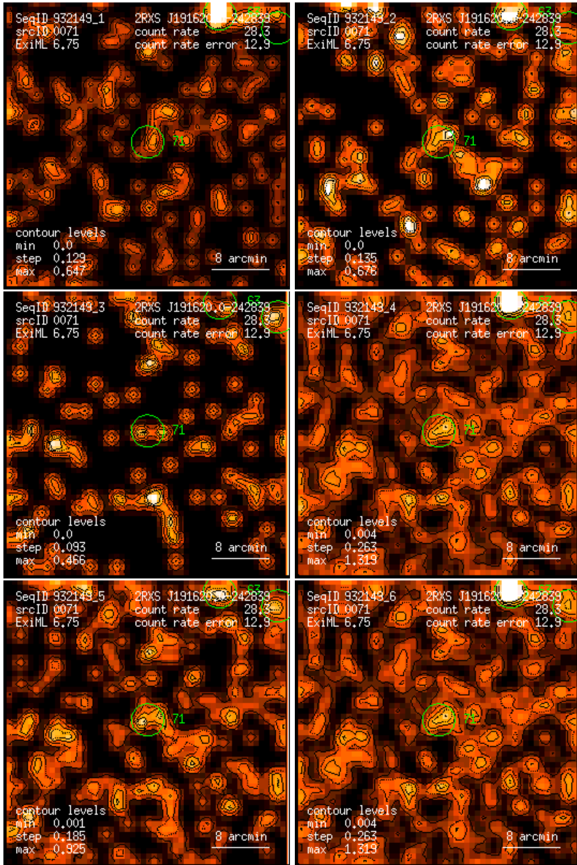
Figure 71: RASS 932149: detection 0071: band rate images, Gaussian filter: (1) PSPC channels 11 – 41, (2) 52 – 90, (3) 91 – 201, (4) 11 – 235, (5) 52 – 201, (6) 11 – 201. Broad band rates in counts/ks. Band rate contour levels in counts/ks/arcmin 2 .
