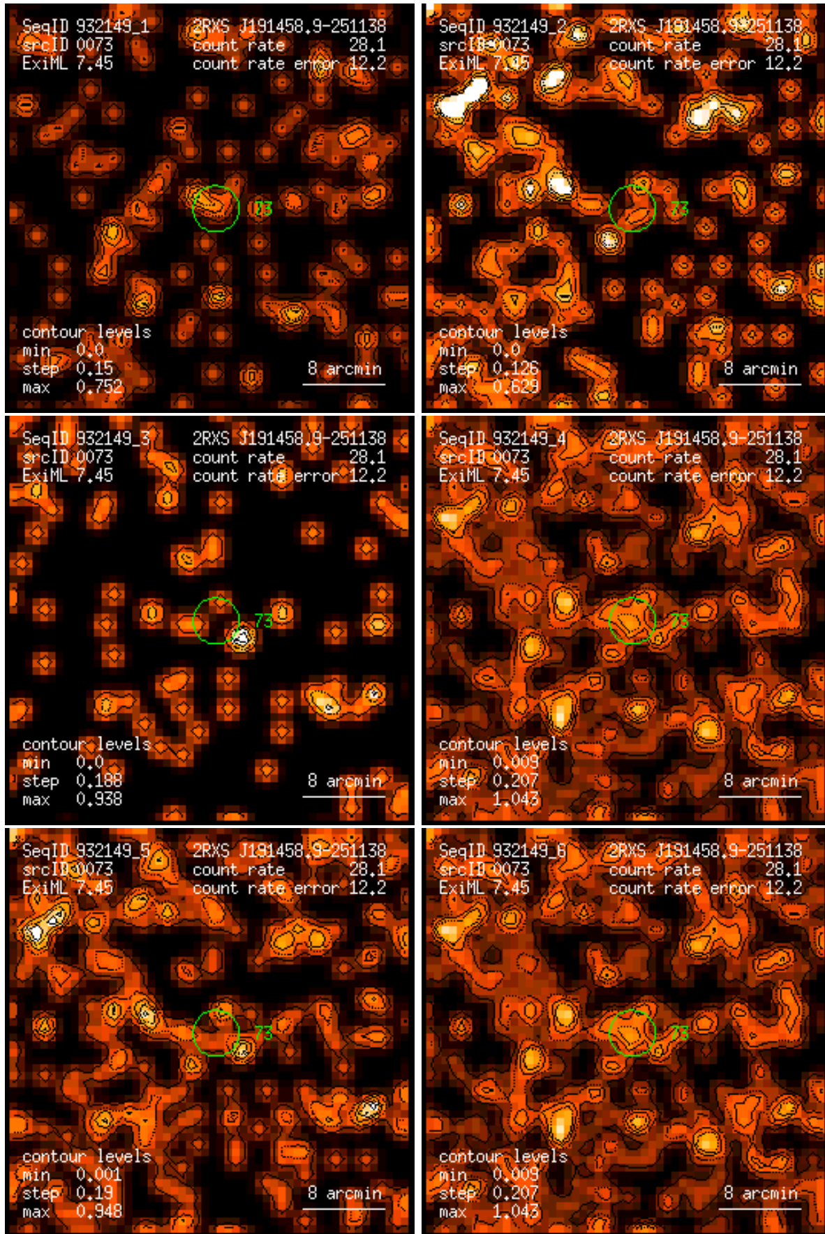
Figure 73: RASS 932149: detection 0073: band rate images, Gaussian filter: (1) PSPC channels 11 – 41, (2) 52 – 90, (3) 91 – 201, (4) 11 – 235, (5) 52 – 201, (6) 11 – 201. Broad band rates in counts/ks. Band rate contour levels in counts/ks/arcmin 2 .
