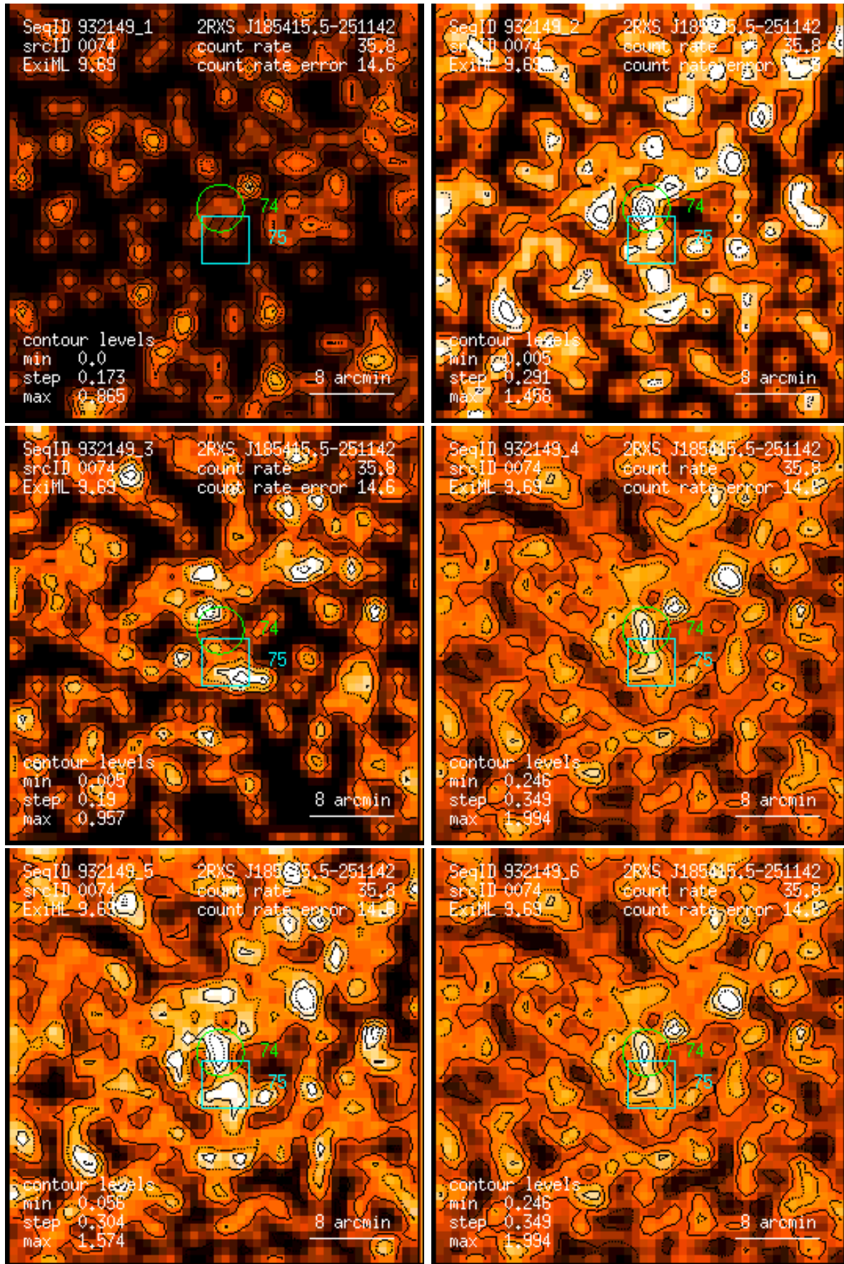
Figure 74: RASS 932149: detection 0074: band rate images, Gaussian filter: (1) PSPC channels 11 – 41, (2) 52 – 90, (3) 91 – 201, (4) 11 – 235, (5) 52 – 201, (6) 11 – 201. Broad band rates in counts/ks. Band rate contour levels in counts/ks/arcmin 2 .
