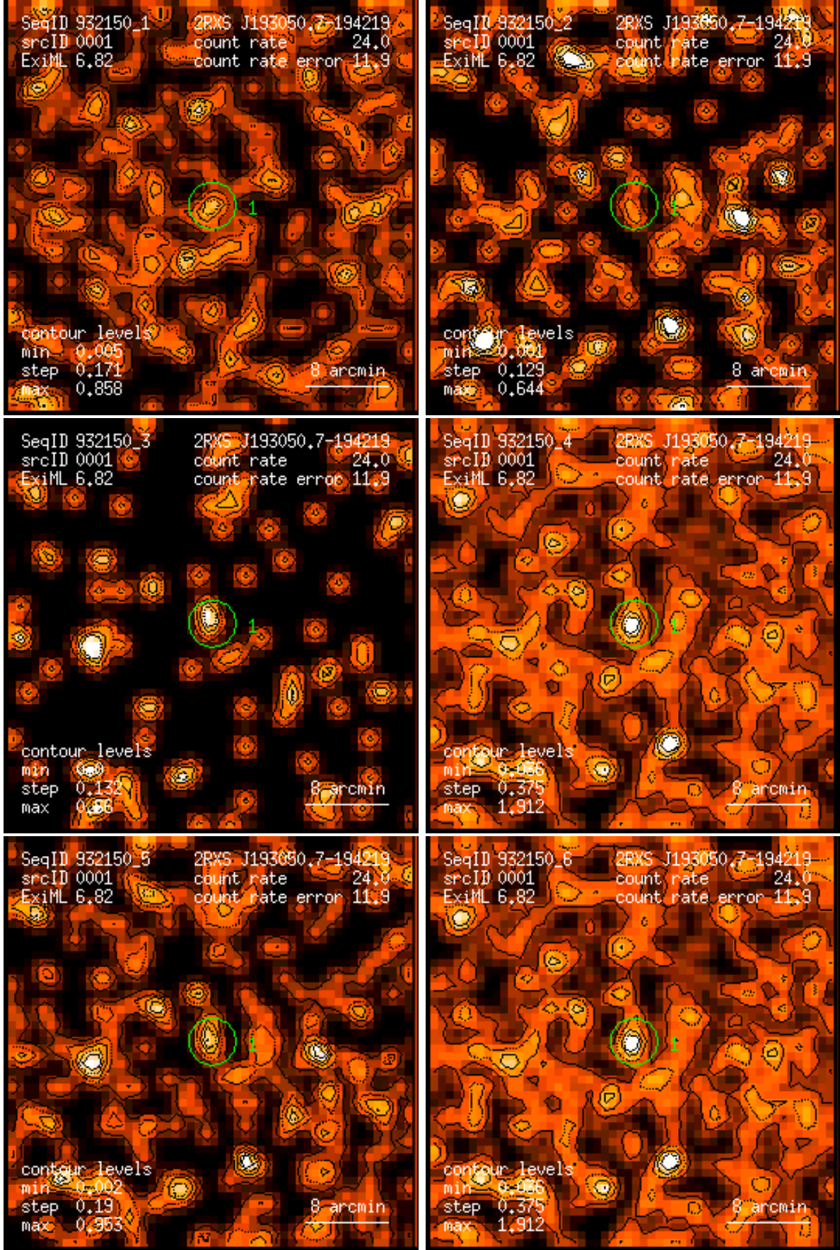
Figure 1: RASS 932150: detection 0001: band rate images, Gaussian filter: (1) PSPC channels 11 – 41, (2) 52 – 90, (3) 91 – 201, (4) 11 – 235, (5) 52 – 201, (6) 11 – 201. Broad band rates in counts/ks. Band rate contour levels in counts/ks/arcmin 2 .
