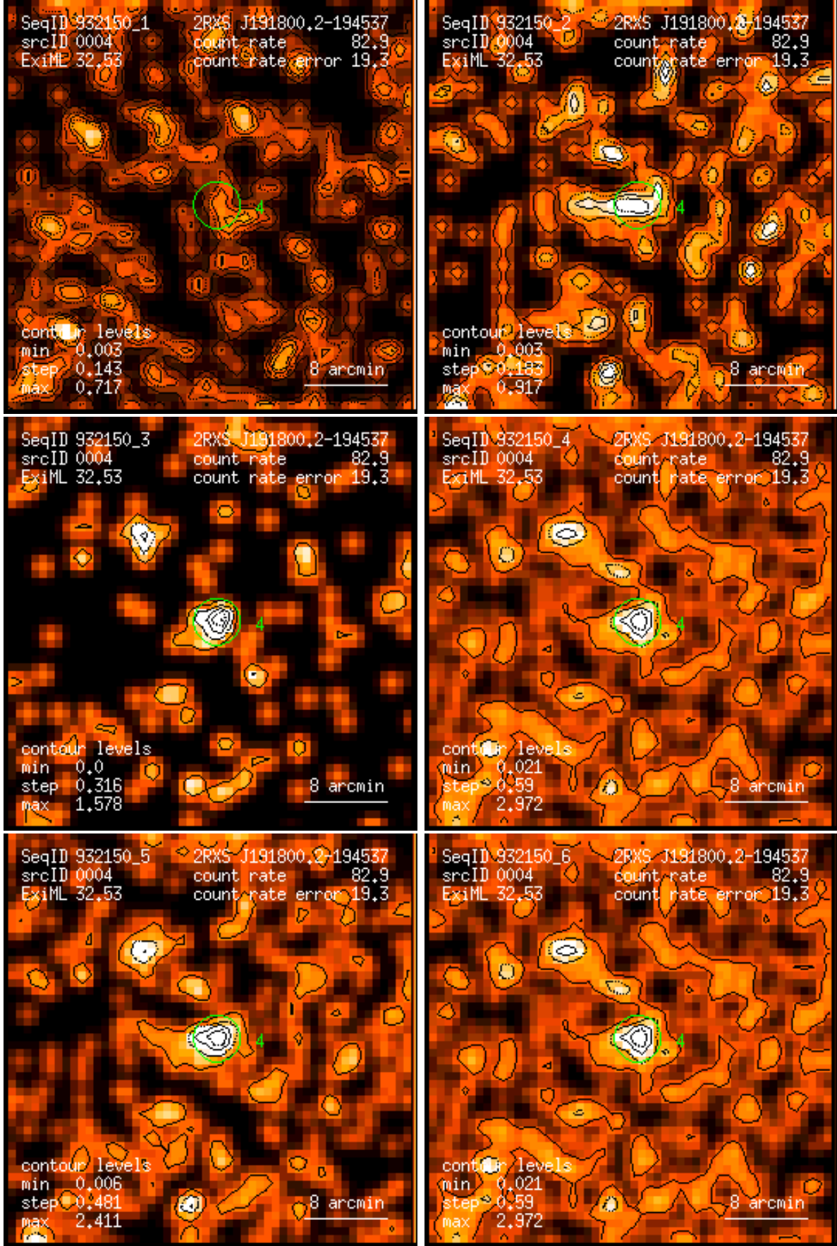
Figure 4: RASS 932150: detection 0004: band rate images, Gaussian filter: (1) PSPC channels 11 – 41, (2) 52 – 90, (3) 91 – 201, (4) 11 – 235, (5) 52 – 201, (6) 11 – 201. Broad band rates in counts/ks. Band rate contour levels in counts/ks/arcmin 2 .
