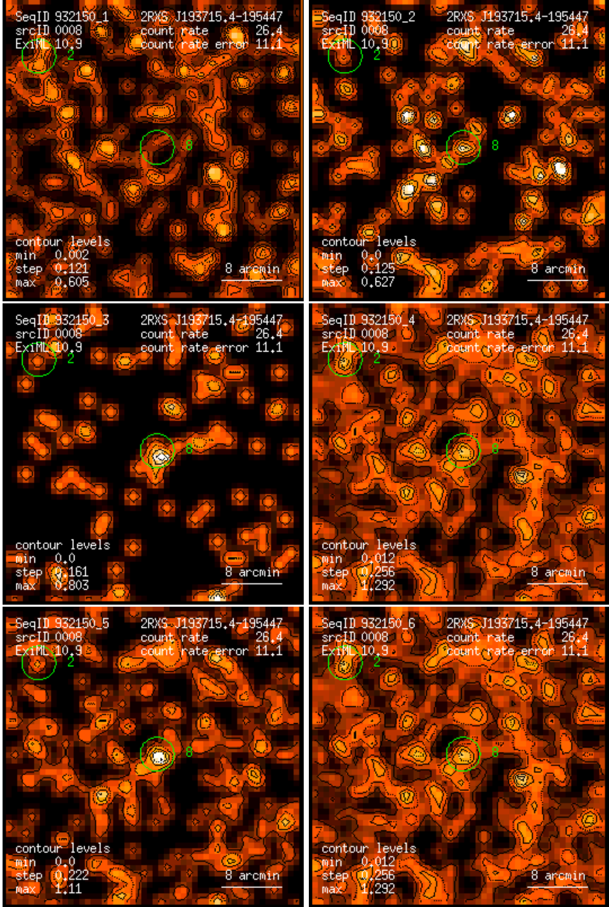
Figure 8: RASS 932150: detection 0008: band rate images, Gaussian filter: (1) PSPC channels 11 – 41, (2) 52 – 90, (3) 91 – 201, (4) 11 – 235, (5) 52 – 201, (6) 11 – 201. Broad band rates in counts/ks. Band rate contour levels in counts/ks/arcmin 2 .
