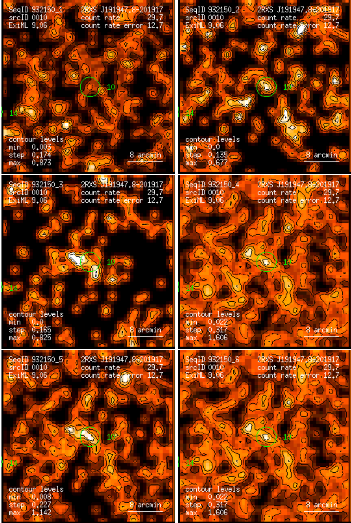
Figure 10: RASS 932150: detection 0010: band rate images, Gaussian filter: (1) PSPC channels 11 – 41, (2) 52 – 90, (3) 91 – 201, (4) 11 – 235, (5) 52 – 201, (6) 11 – 201. Broad band rates in counts/ks. Band rate contour levels in counts/ks/arcmin 2 .
