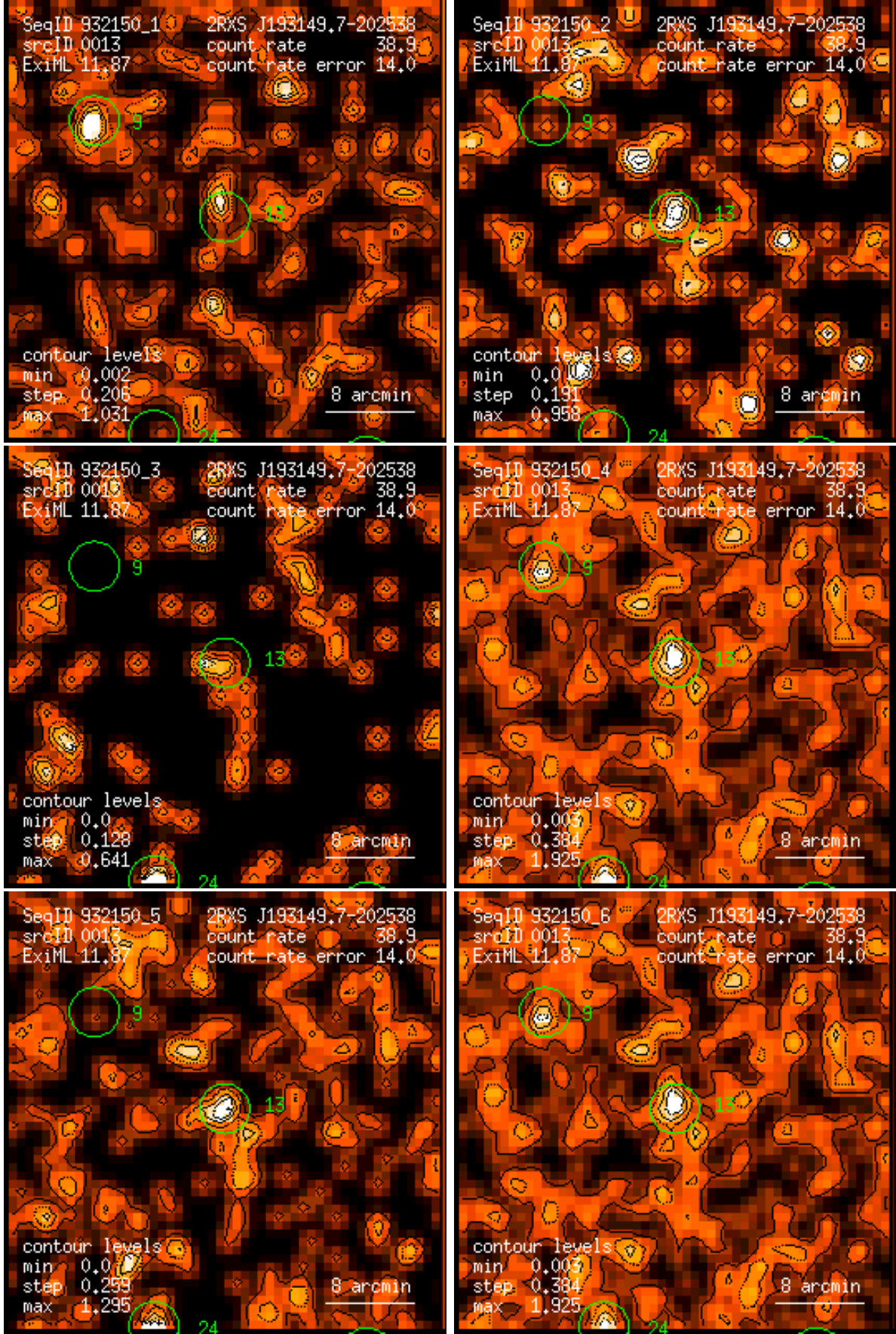
Figure 13: RASS 932150: detection 0013: band rate images, Gaussian filter: (1) PSPC channels 11 – 41, (2) 52 – 90, (3) 91 – 201, (4) 11 – 235, (5) 52 – 201, (6) 11 – 201. Broad band rates in counts/ks. Band rate contour levels in counts/ks/arcmin 2 .
