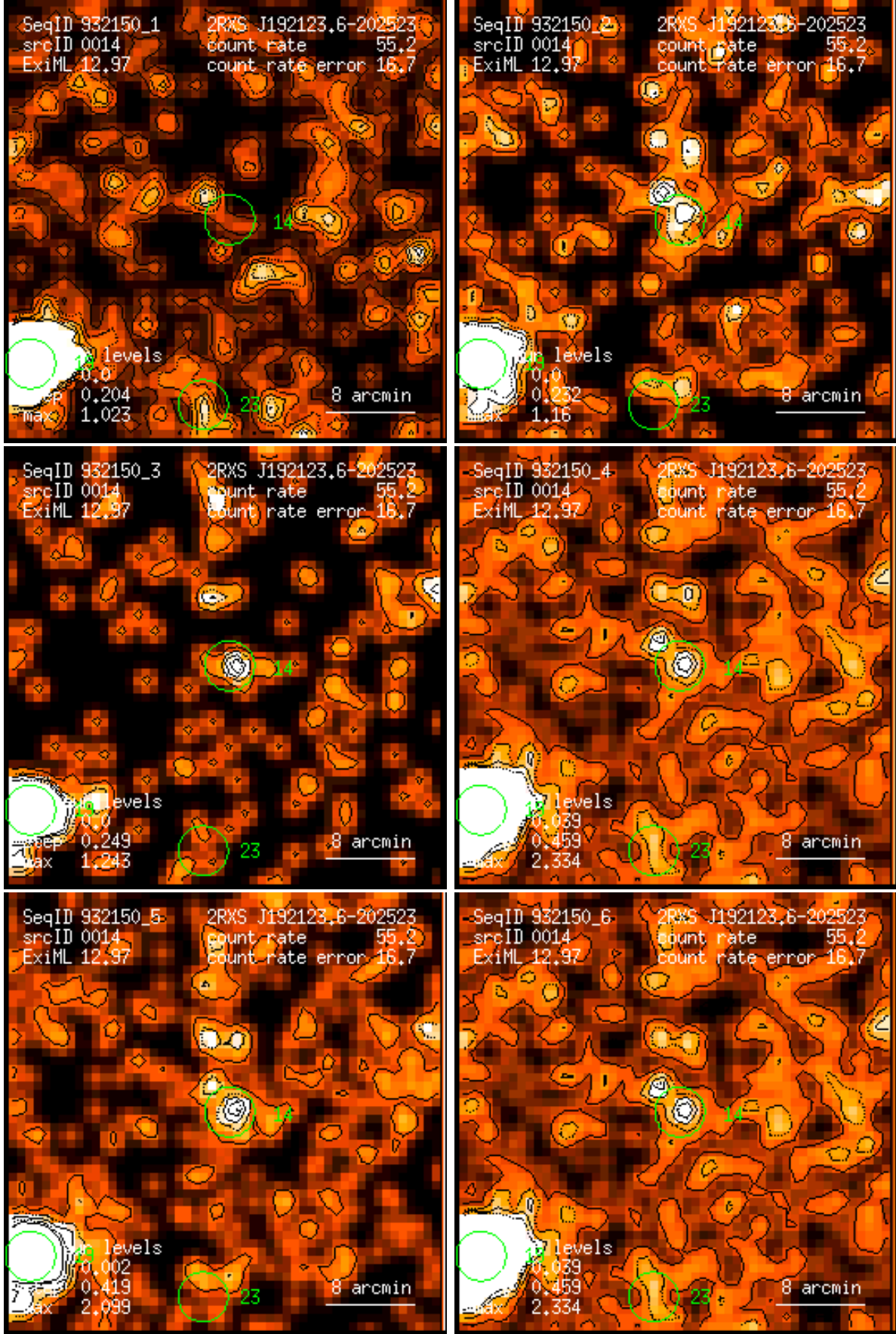
Figure 14: RASS 932150: detection 0014: band rate images, Gaussian filter: (1) PSPC channels 11 – 41, (2) 52 – 90, (3) 91 – 201, (4) 11 – 235, (5) 52 – 201, (6) 11 – 201. Broad band rates in counts/ks. Band rate contour levels in counts/ks/arcmin 2 .
