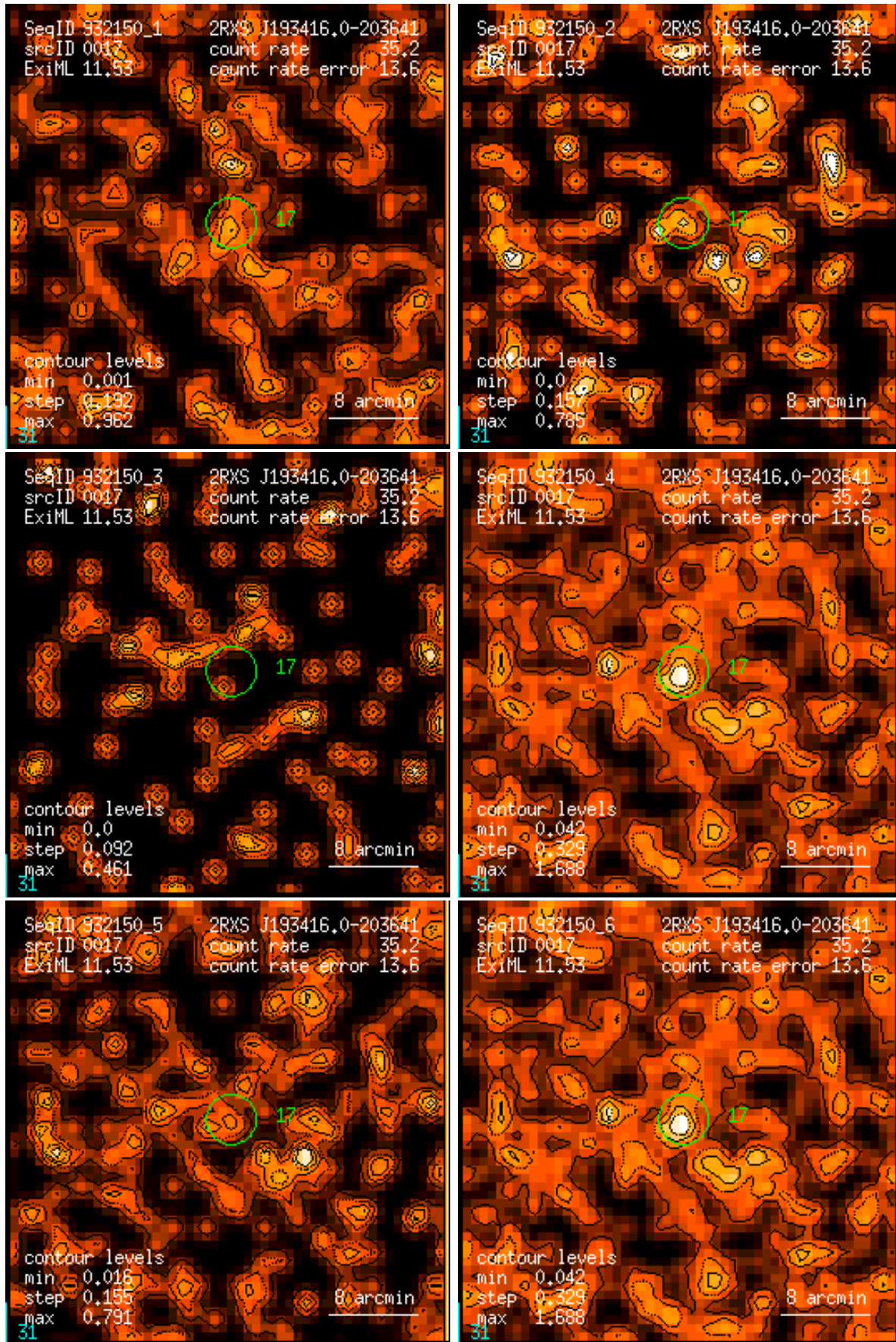
Figure 17: RASS 932150: detection 0017: band rate images, Gaussian filter: (1) PSPC channels 11 – 41, (2) 52 – 90, (3) 91 – 201, (4) 11 – 235, (5) 52 – 201, (6) 11 – 201. Broad band rates in counts/ks. Band rate contour levels in counts/ks/arcmin 2 .
