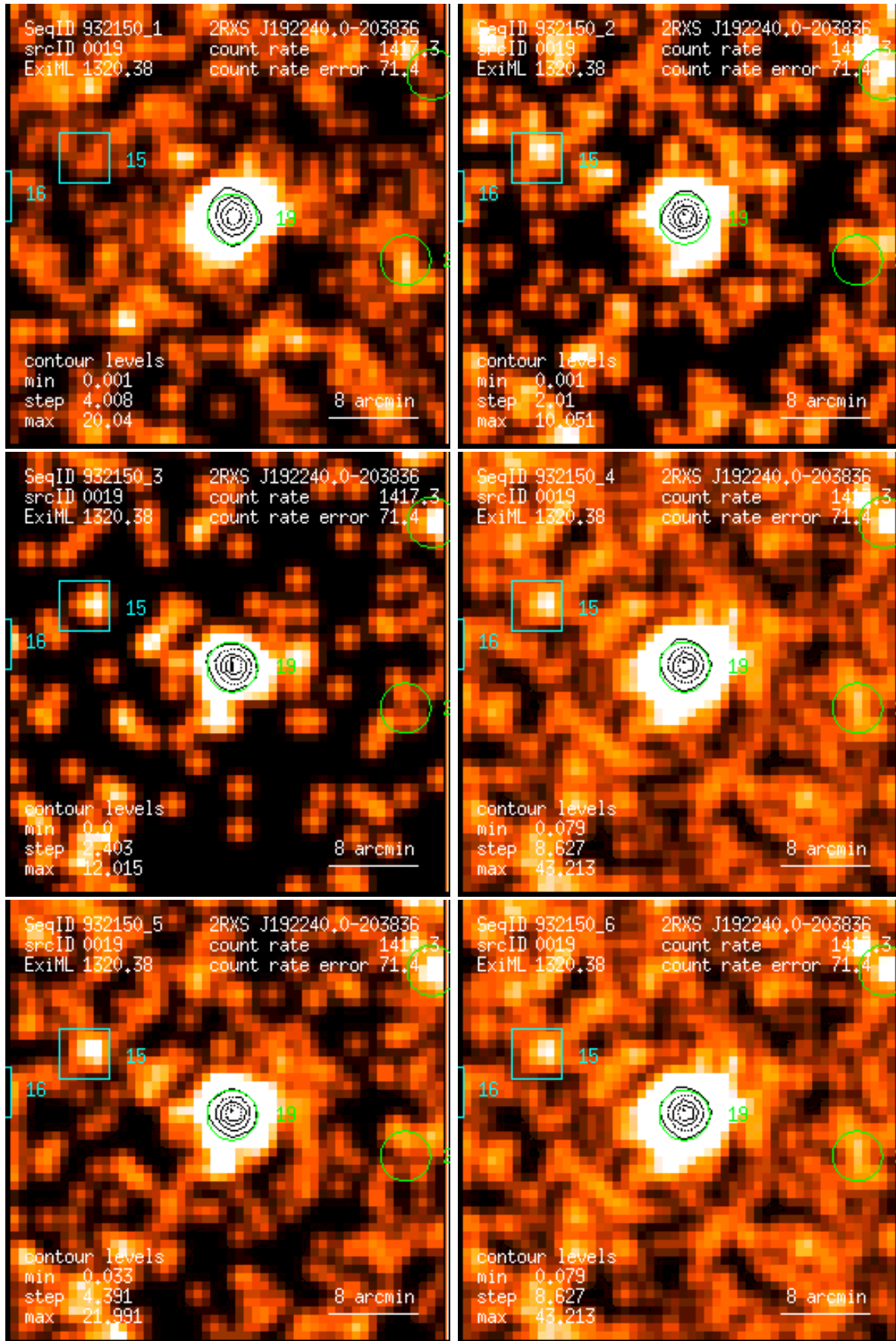
Figure 19: RASS 932150: detection 0019: band rate images, Gaussian filter: (1) PSPC channels 11 – 41, (2) 52 – 90, (3) 91 – 201, (4) 11 – 235, (5) 52 – 201, (6) 11 – 201. Broad band rates in counts/ks. Band rate contour levels in counts/ks/arcmin 2 .
