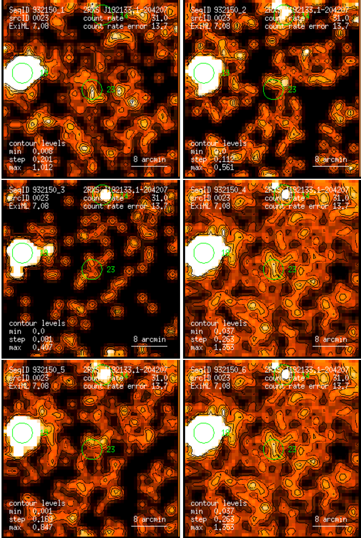
Figure 23: RASS 932150: detection 0023: band rate images, Gaussian filter: (1) PSPC channels 11 – 41, (2) 52 – 90, (3) 91 – 201, (4) 11 – 235, (5) 52 – 201, (6) 11 – 201. Broad band rates in counts/ks. Band rate contour levels in counts/ks/arcmin 2 .
