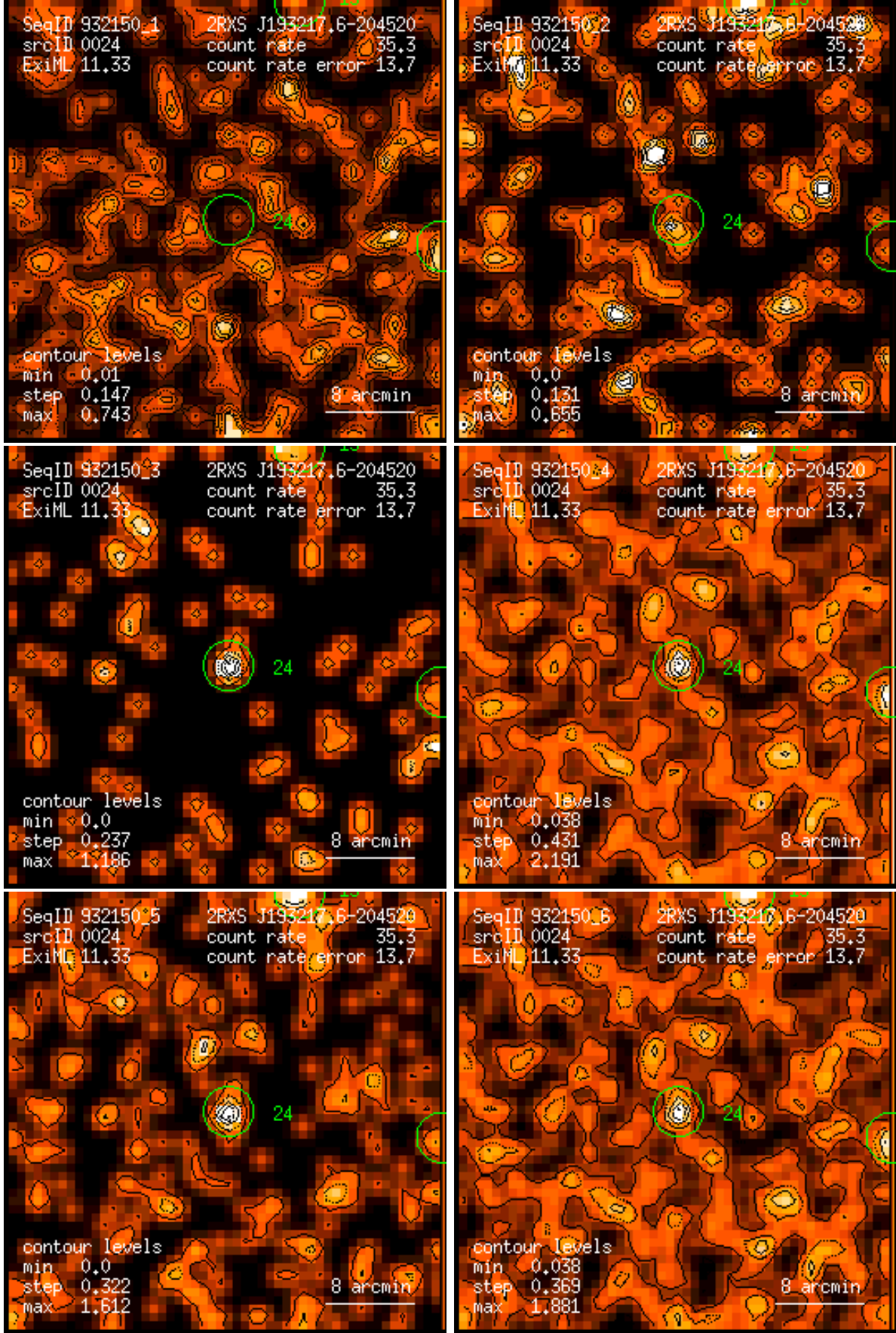
Figure 24: RASS 932150: detection 0024: band rate images, Gaussian filter: (1) PSPC channels 11 – 41, (2) 52 – 90, (3) 91 – 201, (4) 11 – 235, (5) 52 – 201, (6) 11 – 201. Broad band rates in counts/ks. Band rate contour levels in counts/ks/arcmin 2 .
