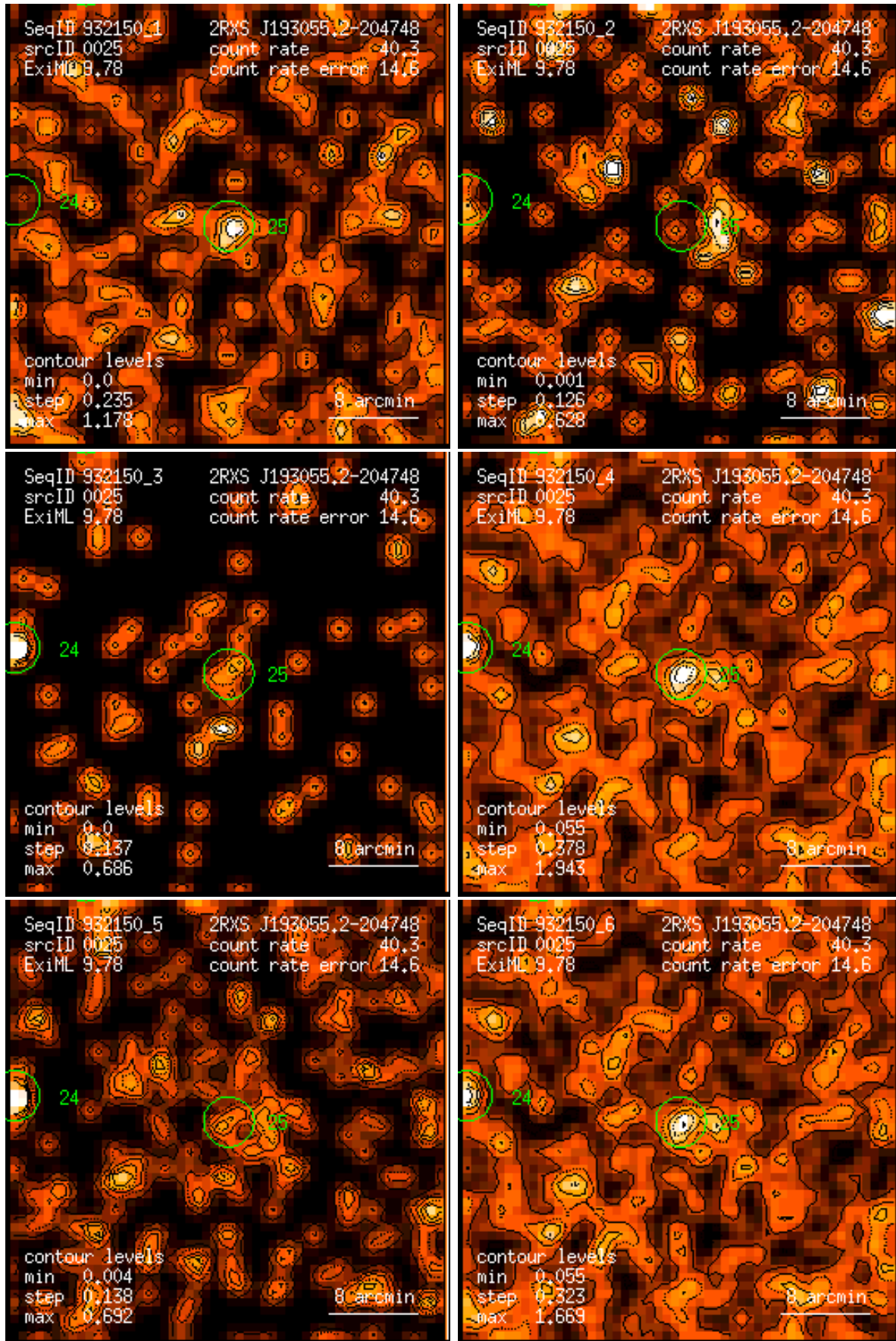
Figure 25: RASS 932150: detection 0025: band rate images, Gaussian filter: (1) PSPC channels 11 – 41, (2) 52 – 90, (3) 91 – 201, (4) 11 – 235, (5) 52 – 201, (6) 11 – 201. Broad band rates in counts/ks. Band rate contour levels in counts/ks/arcmin 2 .
