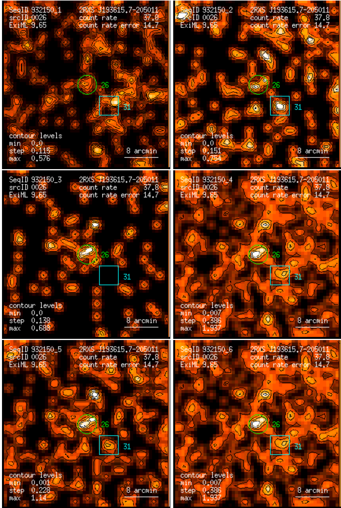
Figure 26: RASS 932150: detection 0026: band rate images, Gaussian filter: (1) PSPC channels 11 – 41, (2) 52 – 90, (3) 91 – 201, (4) 11 – 235, (5) 52 – 201, (6) 11 – 201. Broad band rates in counts/ks. Band rate contour levels in counts/ks/arcmin 2 .
