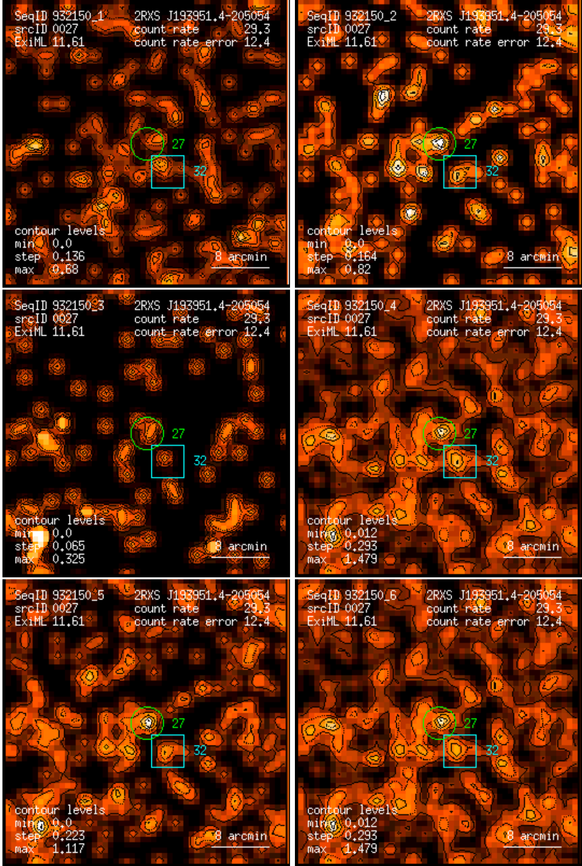
Figure 27: RASS 932150: detection 0027: band rate images, Gaussian filter: (1) PSPC channels 11 – 41, (2) 52 – 90, (3) 91 – 201, (4) 11 – 235, (5) 52 – 201, (6) 11 – 201. Broad band rates in counts/ks. Band rate contour levels in counts/ks/arcmin 2 .
