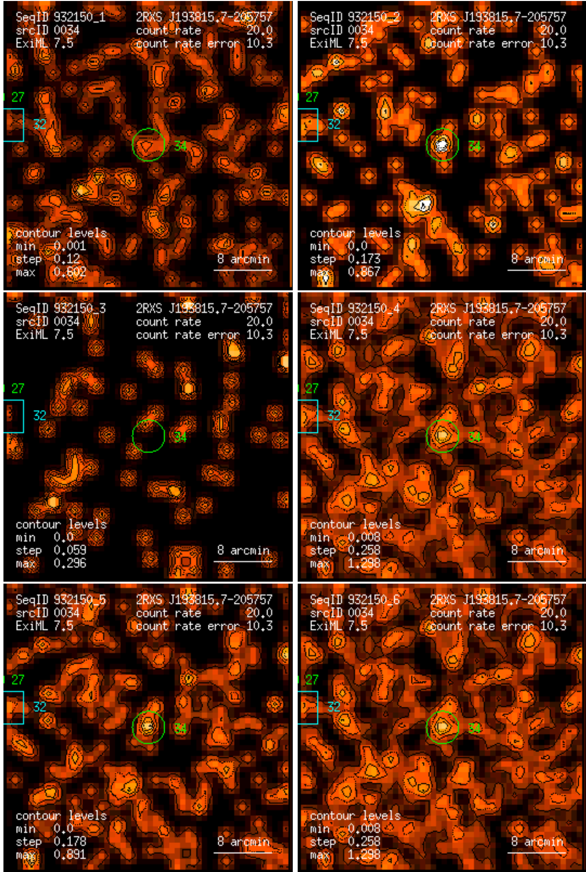
Figure 34: RASS 932150: detection 0034: band rate images, Gaussian filter: (1) PSPC channels 11 – 41, (2) 52 – 90, (3) 91 – 201, (4) 11 – 235, (5) 52 – 201, (6) 11 – 201. Broad band rates in counts/ks. Band rate contour levels in counts/ks/arcmin 2 .
