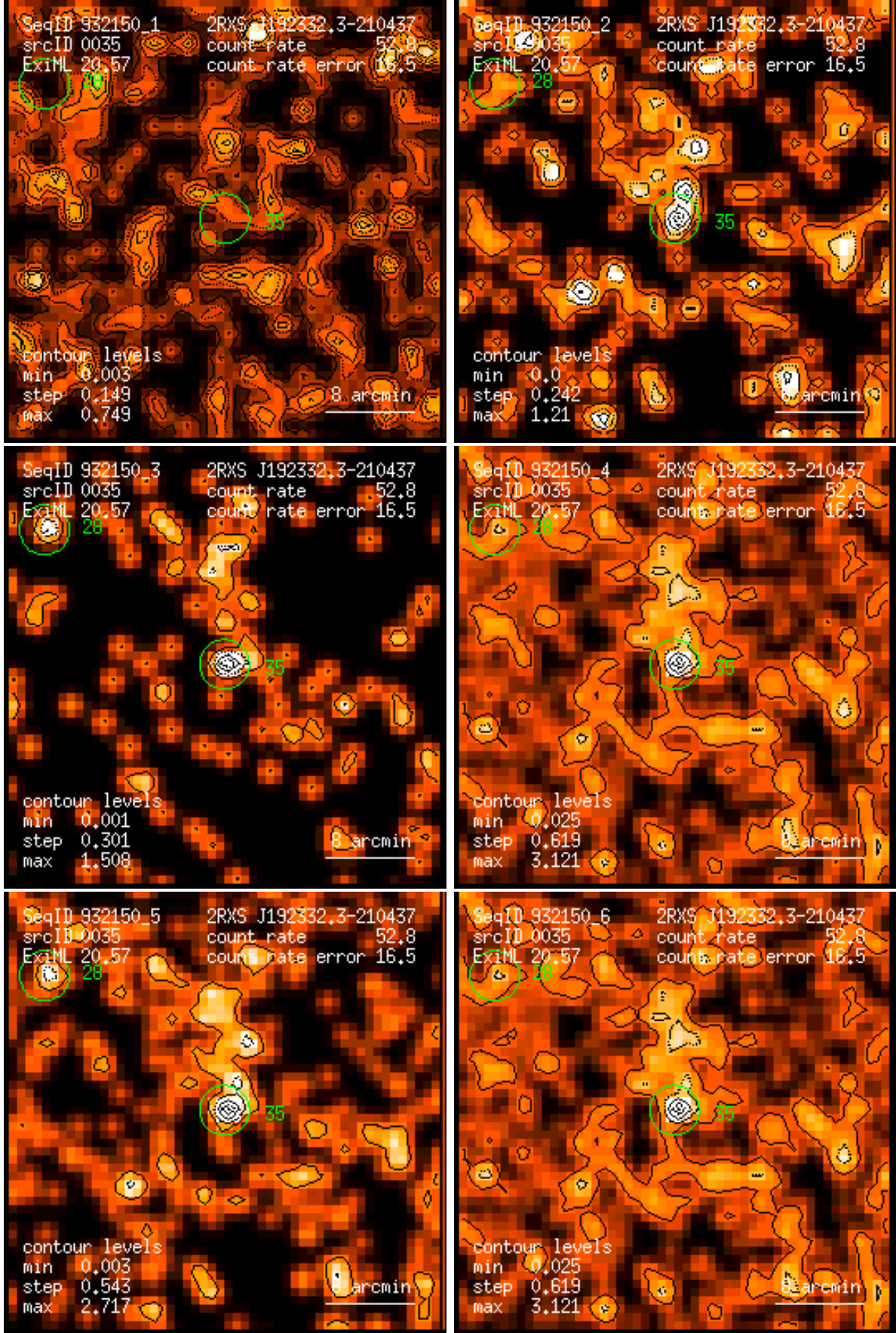
Figure 35: RASS 932150: detection 0035: band rate images, Gaussian filter: (1) PSPC channels 11 – 41, (2) 52 – 90, (3) 91 – 201, (4) 11 – 235, (5) 52 – 201, (6) 11 – 201. Broad band rates in counts/ks. Band rate contour levels in counts/ks/arcmin 2 .
